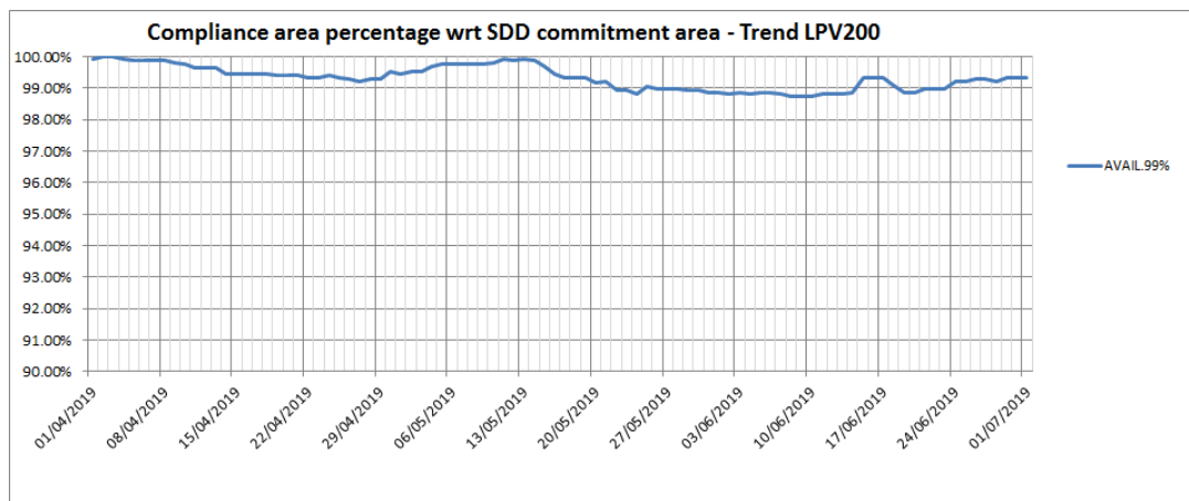
Figure 21 – EGNOS LPV-200 availability compliance trend
