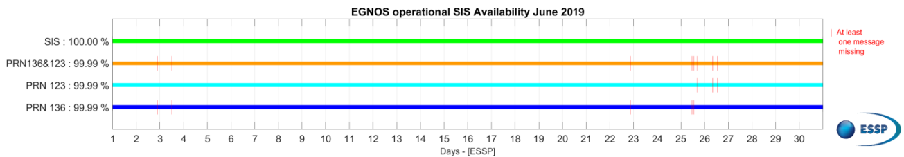
Figure 1 – EGNOS SIS & PRN Availability for June 2019.
