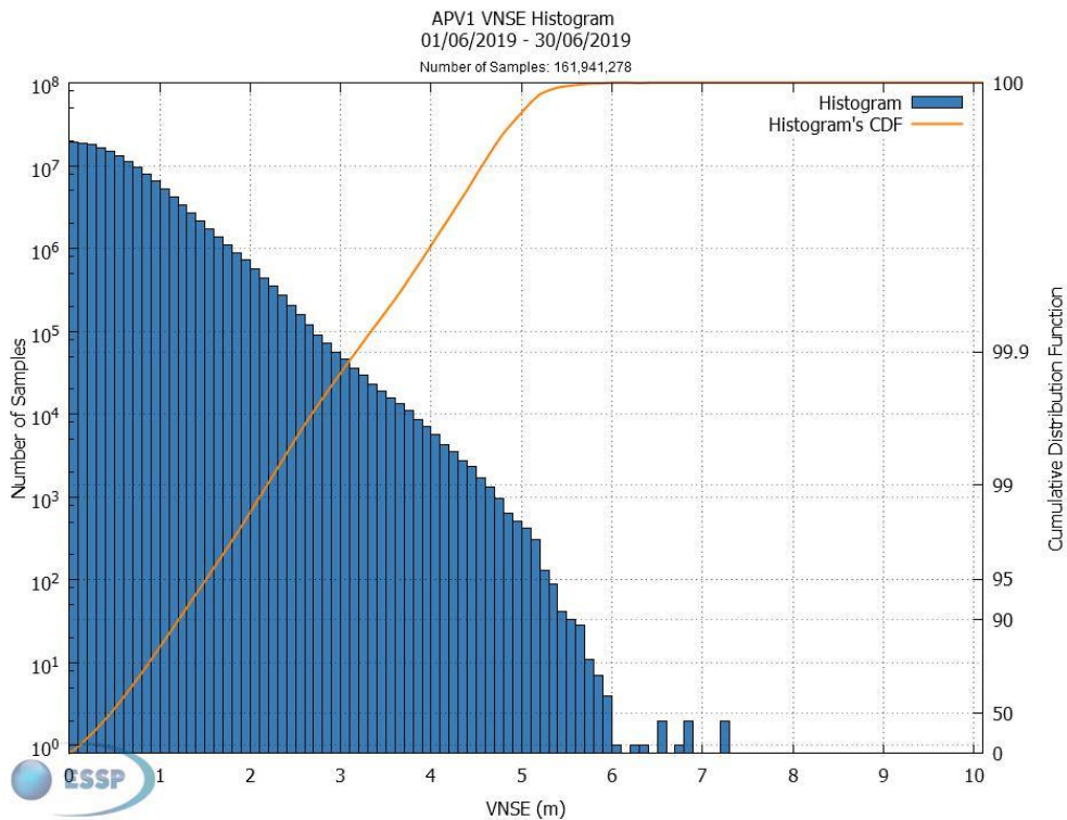
Figure 17 – EGNOS APV-I VNSE Histogram and Cumulative Probability
