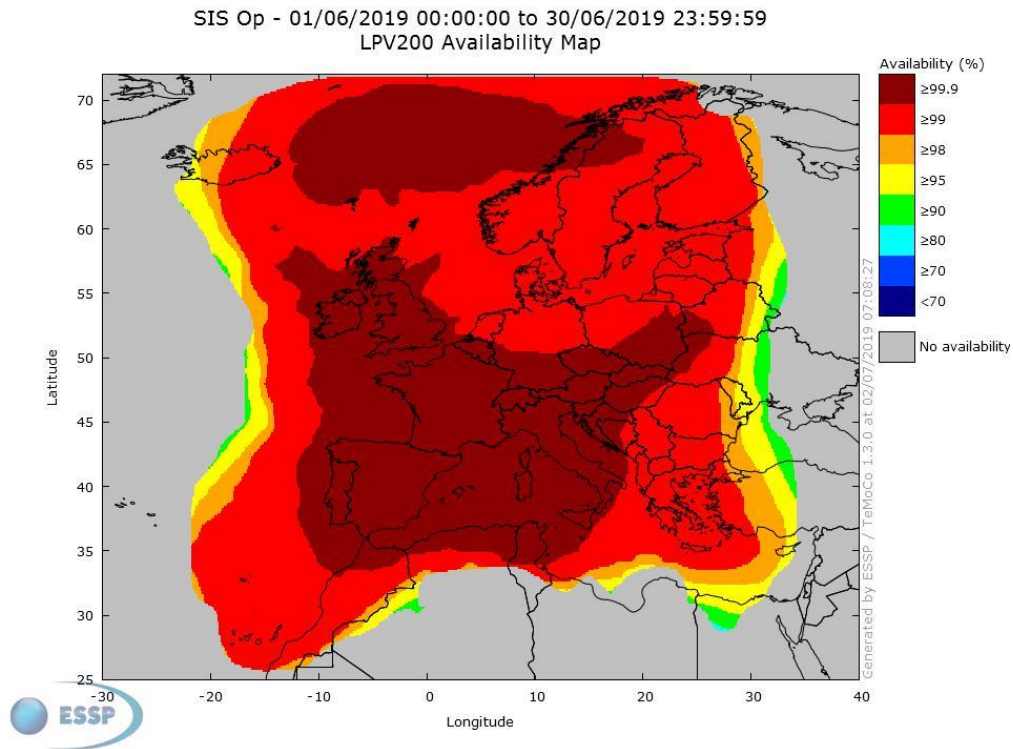
Figure 20 – EGNOS LPV-200 Availability
