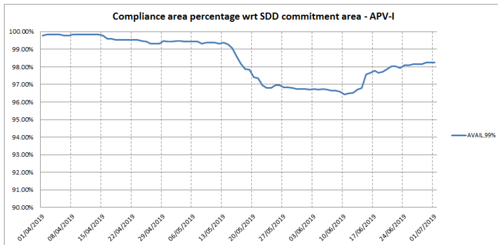
Figure 12 – EGNOS APV-I availability compliance trend
