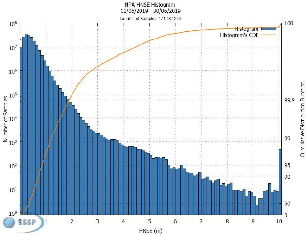
Figure 10 – EGNOS NPA HNSE Histogram and Cumulative Probability
