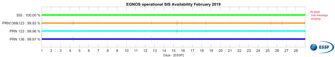
Figure 1 – EGNOS SIS & PRN Availability for February 2019.
