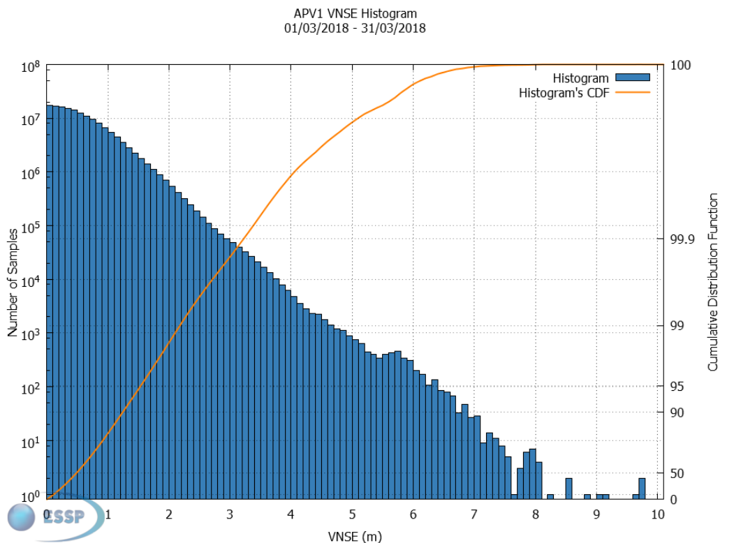
Figure 17 – EGNOS APV-I VNSE Histogram and Cumulative Probability
