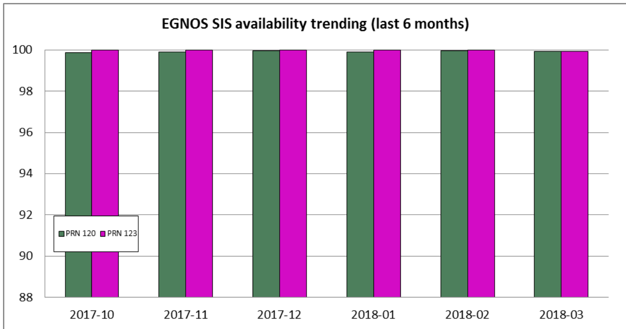
Figure 1 – EGNOS SIS & PRN Availability for March 2018.
