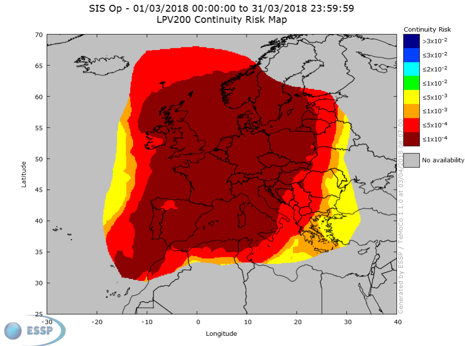
Figure 22 – EGNOS LPV-200 Continuity 2
