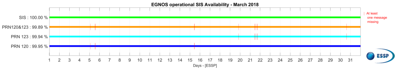
Figure 1 – EGNOS SIS & PRN Availability for March 2018.
