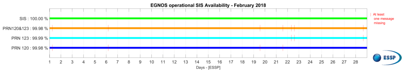
Figure 1 – EGNOS SIS & PRN Availability for February 2018.
