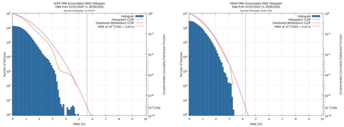
Figure 42 – Extrapolated LPV200 VNSE at 10-7/150s in SOF (left) & SWA (right)
