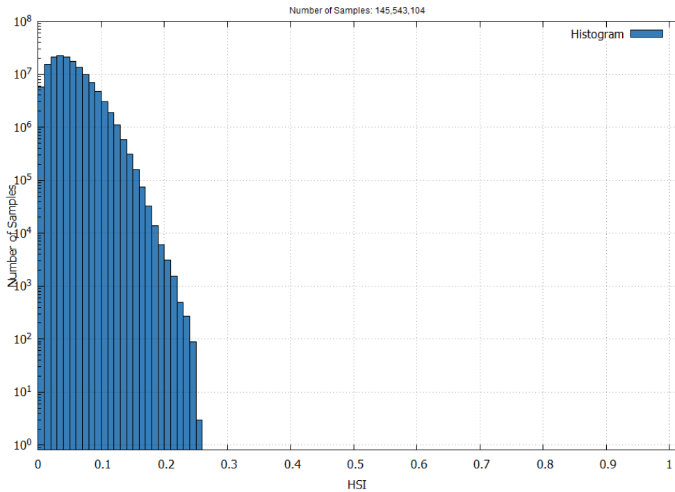
Figure 13 – EGNOS APV-I Horizontal Safety Index in July 2026
