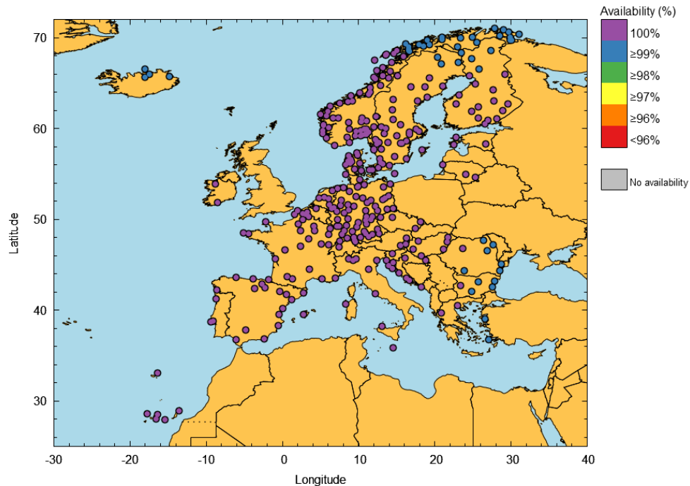
Figure 17 – EGNOS APV-I Availability at airports in July 2026
