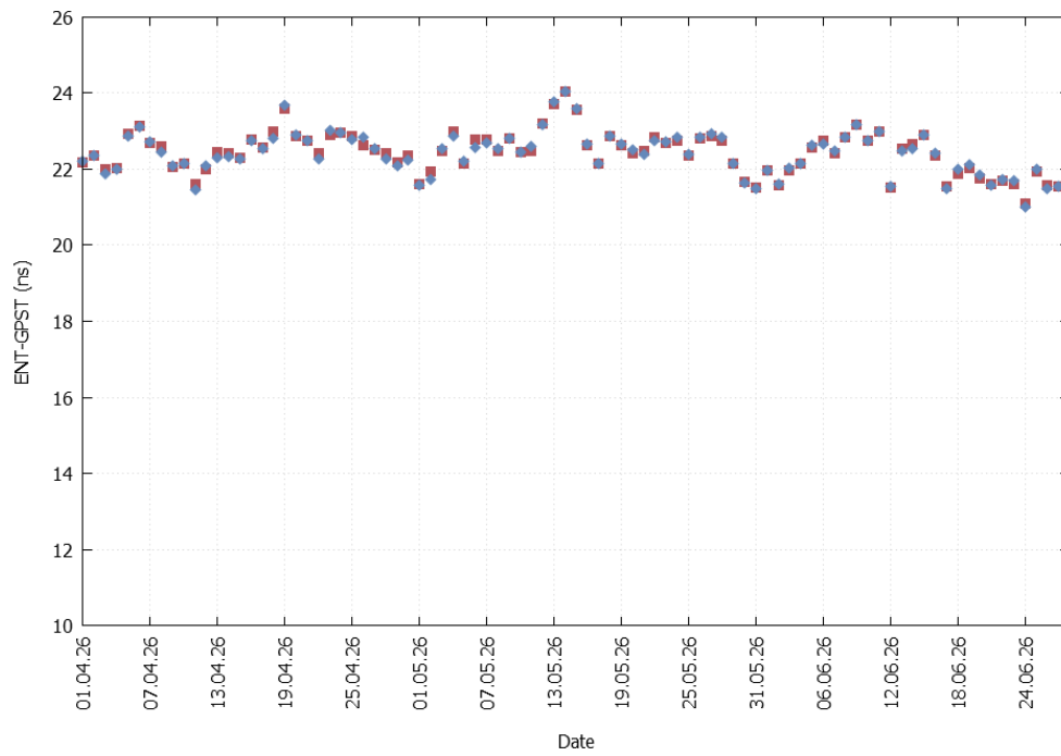
Figure 30 – ENT-GPS offset evolution from April 2026 to June 2026 (red PRN 121; blue PRN 136)
