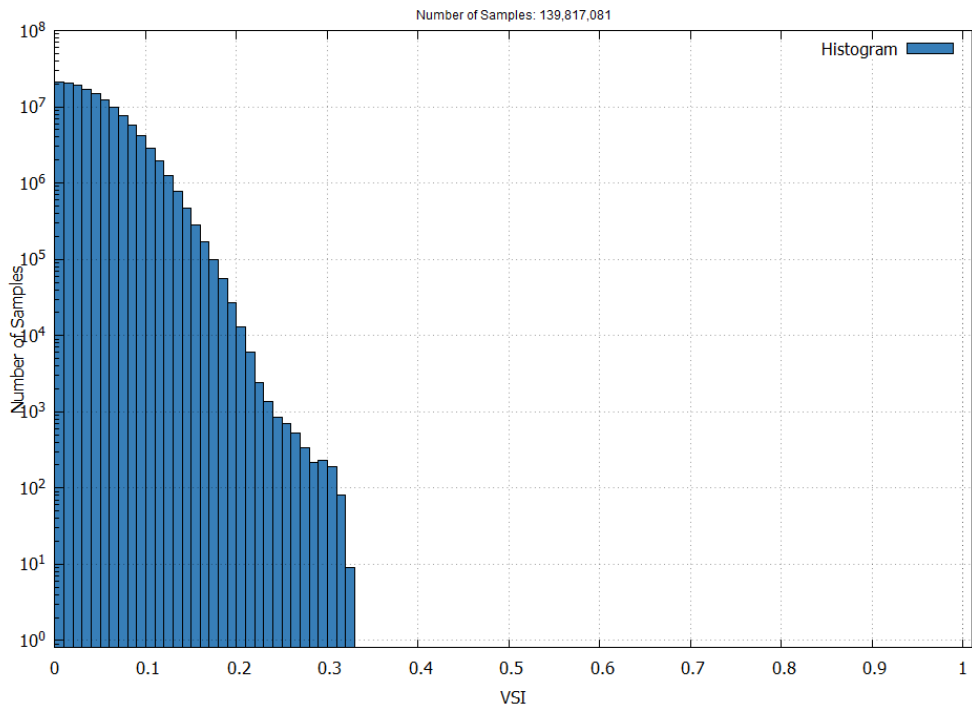
Figure 23 – EGNOS LPV-200 Vertical Safety Index in July 2026
