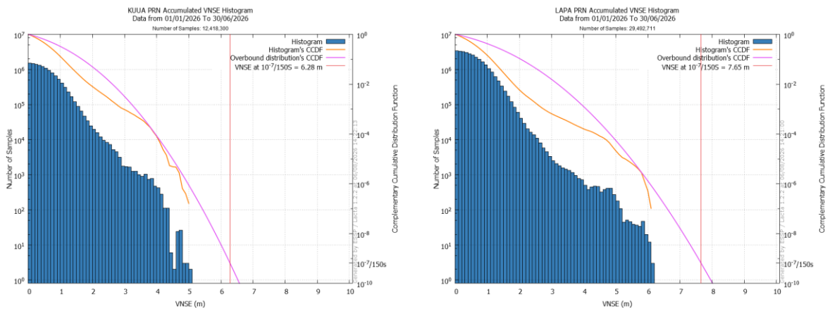
Figure 38 – Extrapolated LPV200 VNSE at 10-7/150s in KUU (left) & LAP (right)
