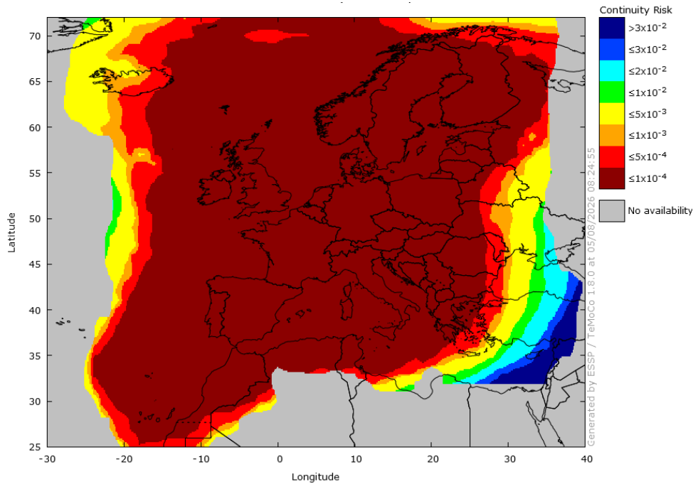
Figure 21 – EGNOS LPV-200 Continuity 2 in July 2026
