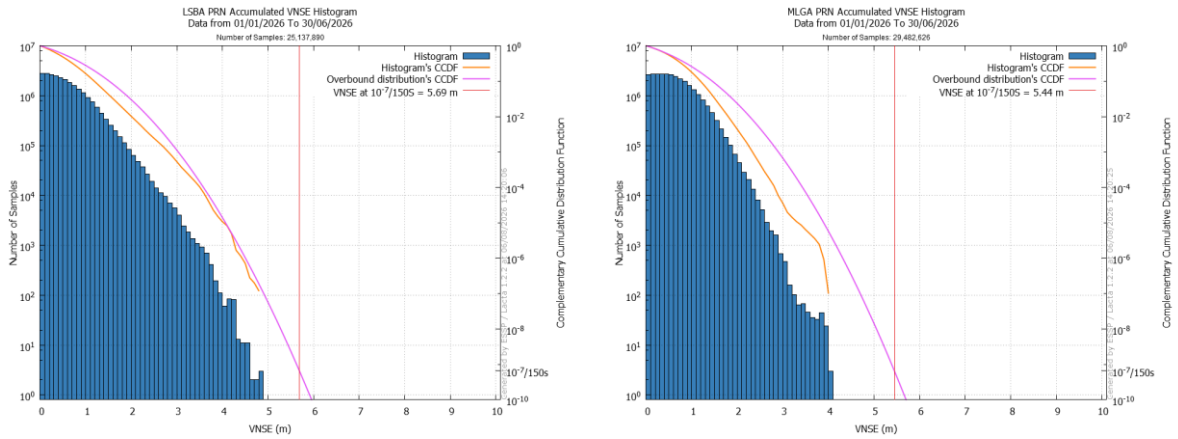
Figure 39 – Extrapolated LPV200 VNSE at 10-7/150s in LSB (left) & MLG (right)
