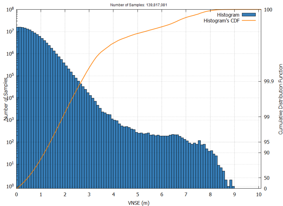
Figure 25 – EGNOS LPV-200 VNSE Histogram and Cumulative Probability in July 2026
