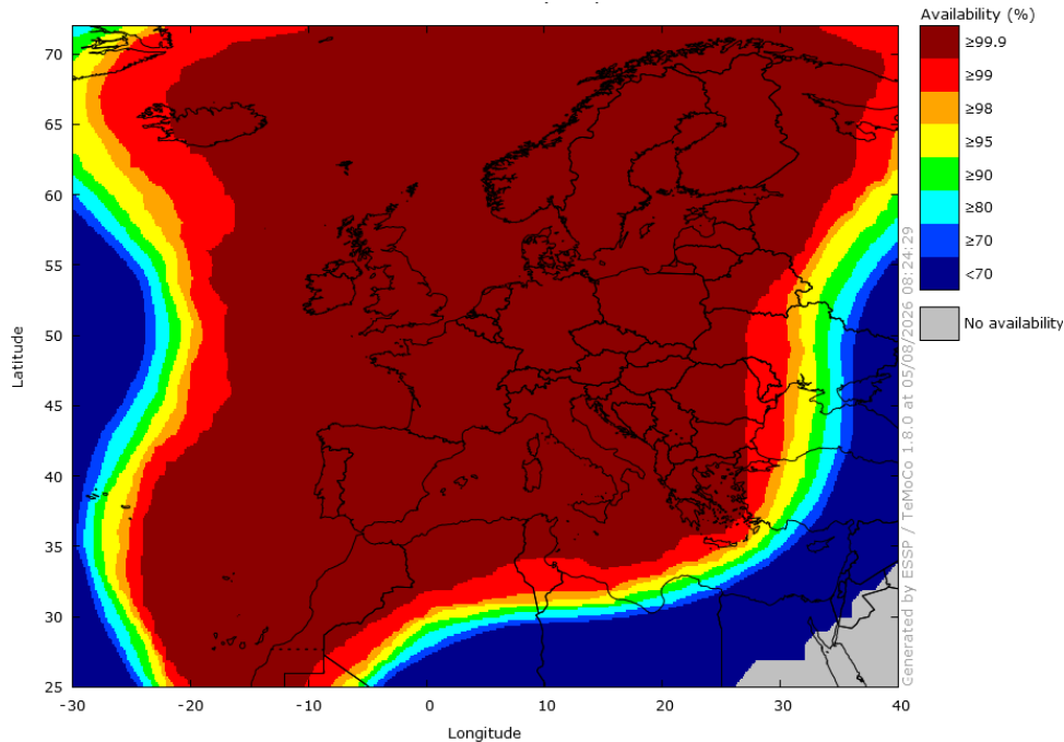
Figure 10 – EGNOS APV-I Availability in July 2026
