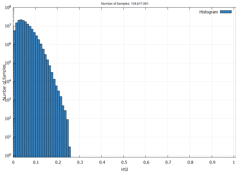
Figure 22 – EGNOS LPV-200 Horizontal Safety Index in July 2026
