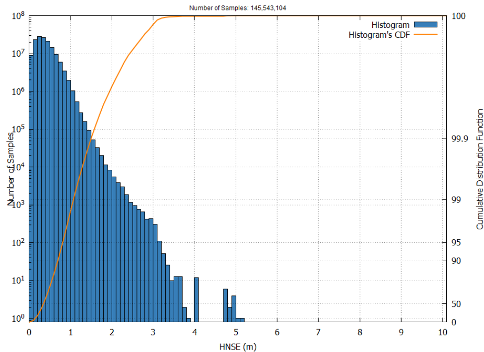
Figure 15 – EGNOS APV-I HNSE Histogram and Cumulative Probability in July 2026
