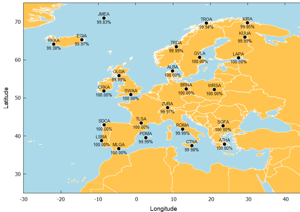
Figure 5 – EGNOS Open Service Availability at reference stations in July 2026
