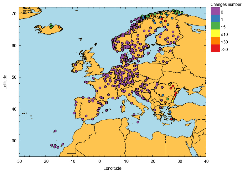
Figure 18 – EGNOS APV-I outages in July 2026
