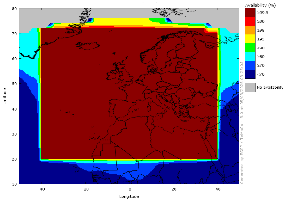
Figure 6 – EGNOS NPA Availability in July 2026
