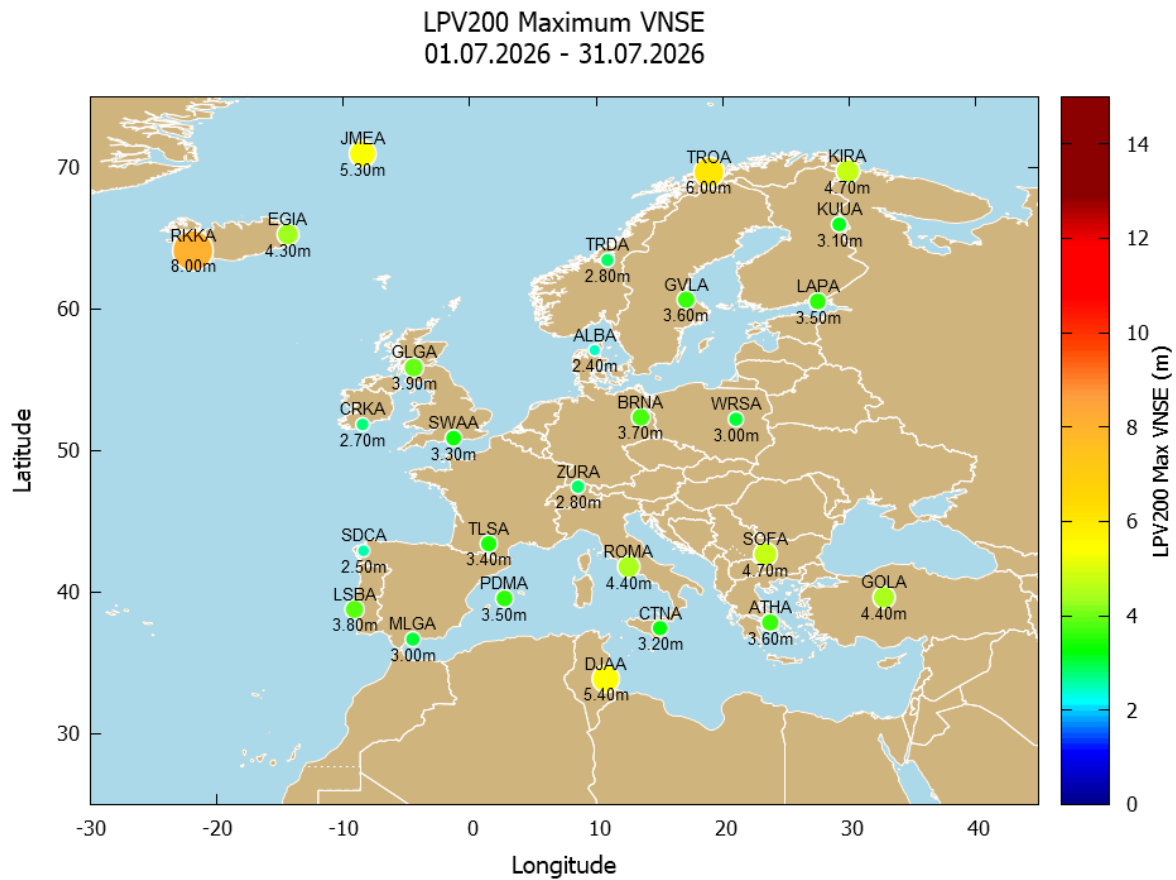
Figure 26 – EGNOS LPV-200 VNSE Maximum Values
