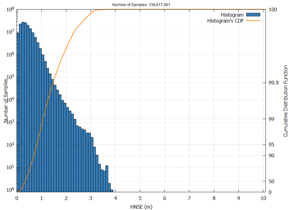
Figure 24 – EGNOS LPV-200 HNSE Histogram and Cumulative Probability in July 2026
