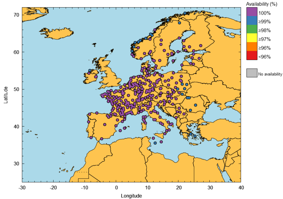
Figure 27 – EGNOS LPV-200 Availability at airports in July 2026
