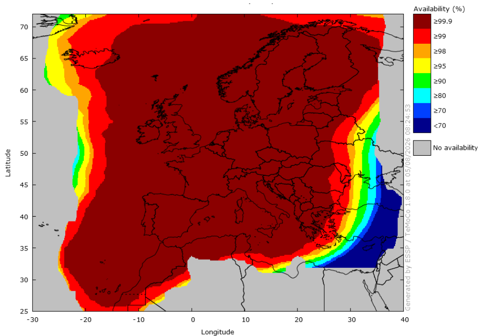
Figure 19 – EGNOS LPV-200 Availability in July 2026
