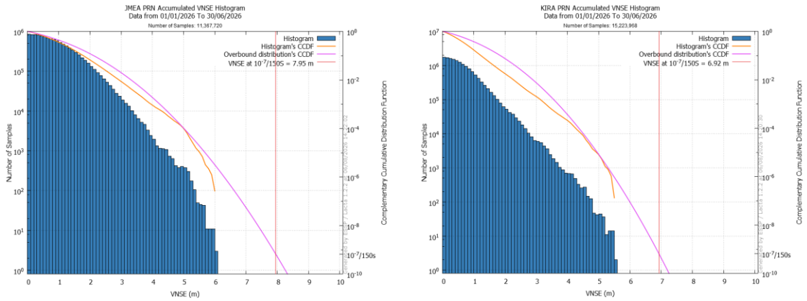
Figure 37 – Extrapolated LPV200 VNSE at 10-7/150s in JME (left) & KIR (right)
