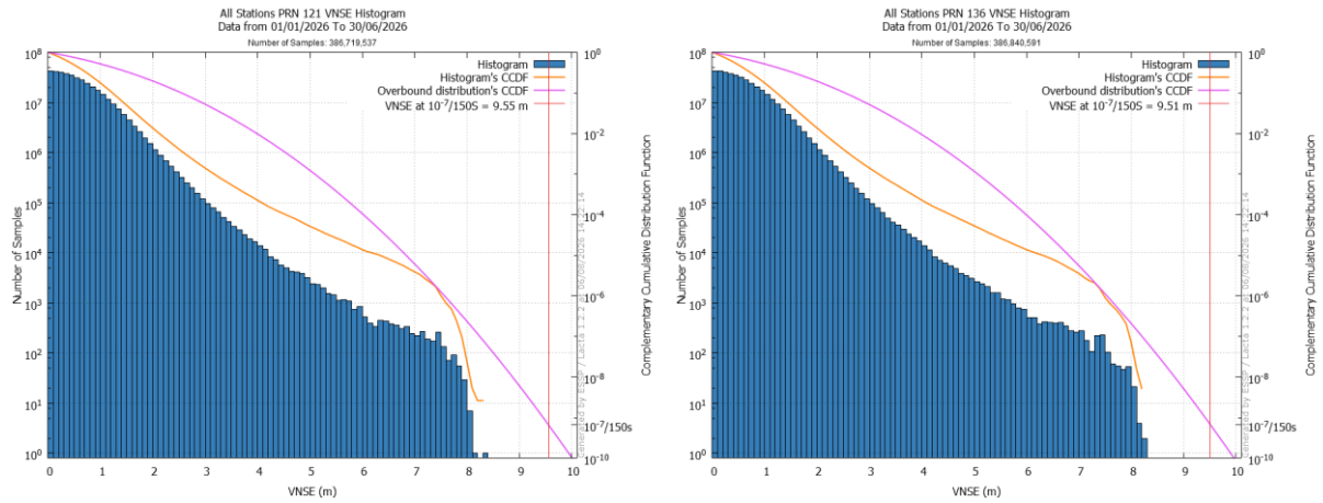
Figure 46 – Extrapolated LPV200 VNSE at 10-7/150s - all RIMS - PRN121 (left) and PRN136 (right)
