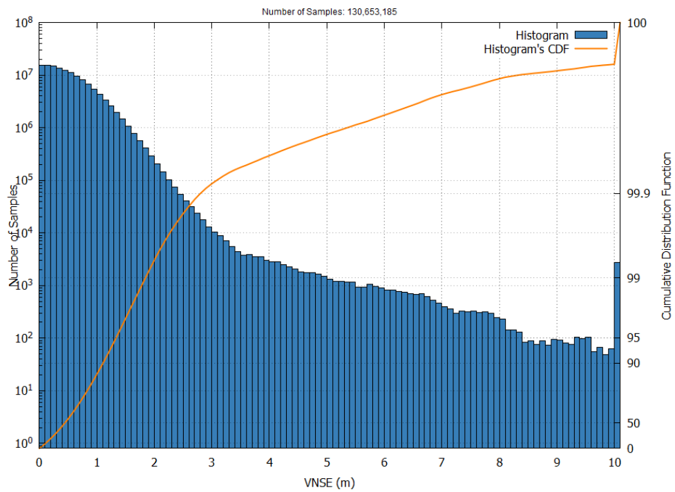
Figure 4 – EGNOS Open Service VNSE Histogram and Cumulative Probability in July 2026
