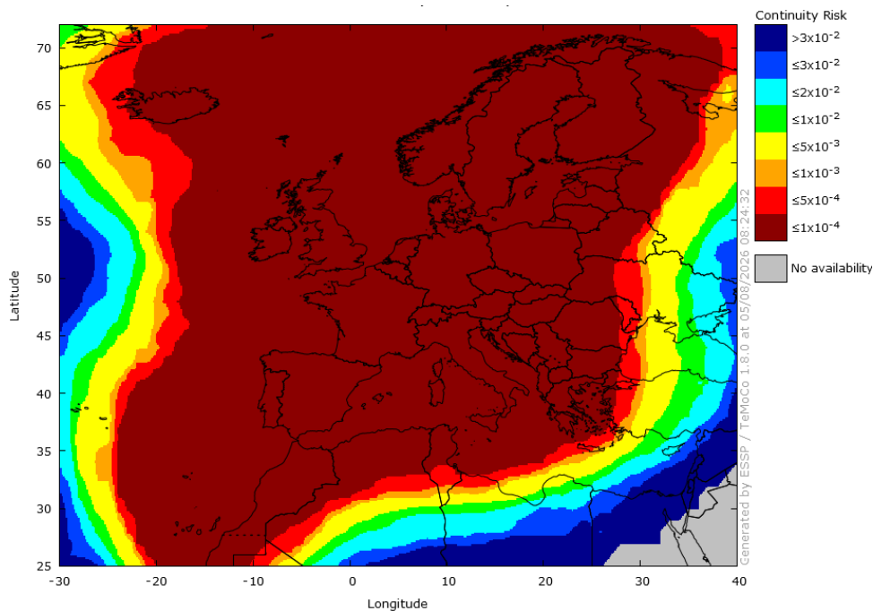
Figure 12 – EGNOS APV-I Continuity in July 2026
