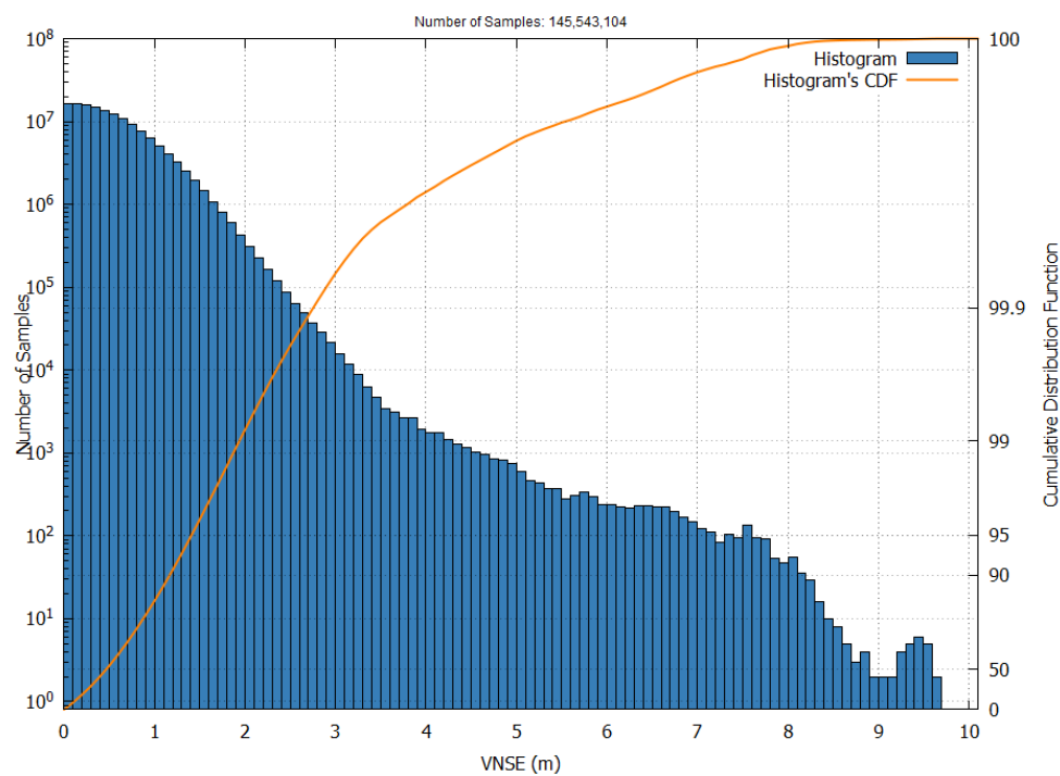
Figure 16 – EGNOS APV-I VNSE Histogram and Cumulative Probability in July 2026
