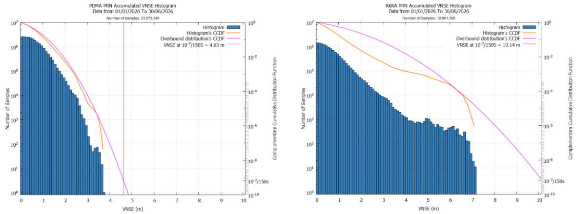
Figure 40 – Extrapolated LPV200 VNSE at 10-7/150s in PDM (left) & RKK (right)
