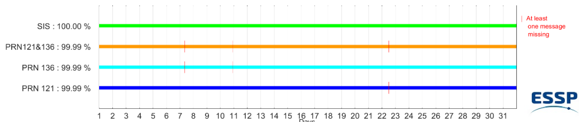
Figure 1 - EGNOS SIS & PRN Availability for July 2026
