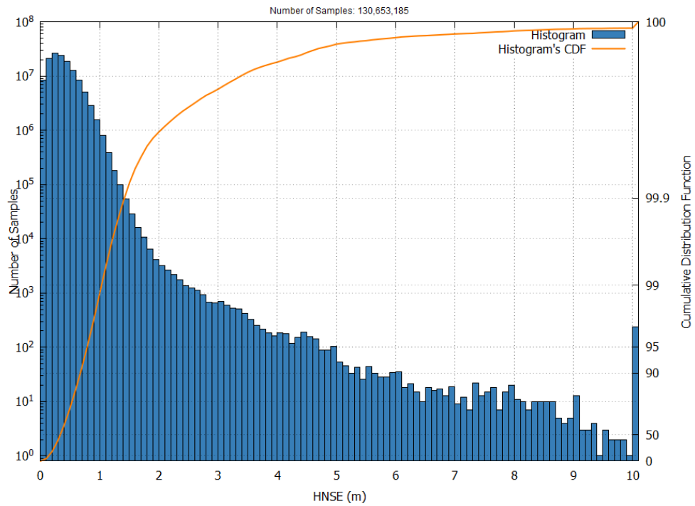
Figure 3 – EGNOS Open Service HNSE Histogram and Cumulative Probability in July 2026
