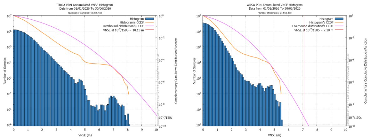
Figure 44 – Extrapolated LPV200 VNSE at 10-7/150s in TRO (left) & WRS (right)
