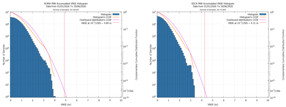
Figure 41 – Extrapolated LPV200 VNSE at 10-7/150s in ROM (left) & SDC (right)
