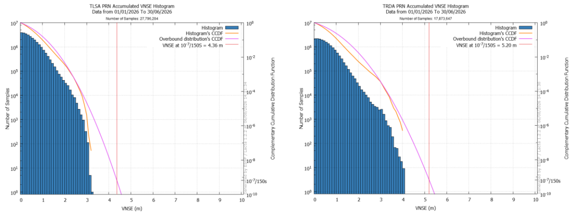
Figure 43 – Extrapolated LPV200 VNSE at 10-7/150s in TLS (left) & TRD (right)
