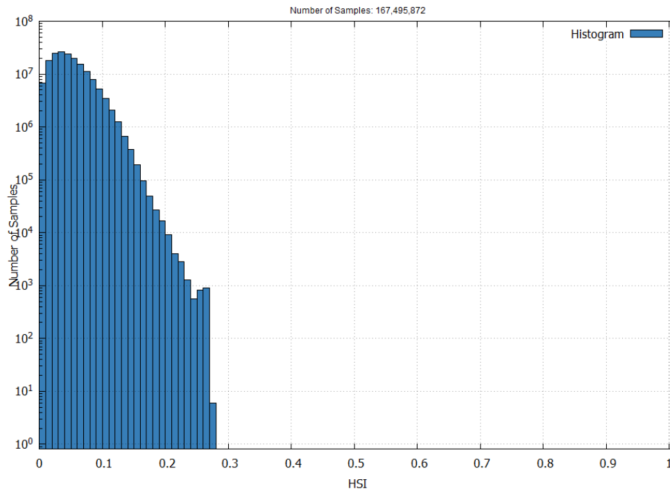
Figure 8 – EGNOS NPA Horizontal Safety Index in July 2026
