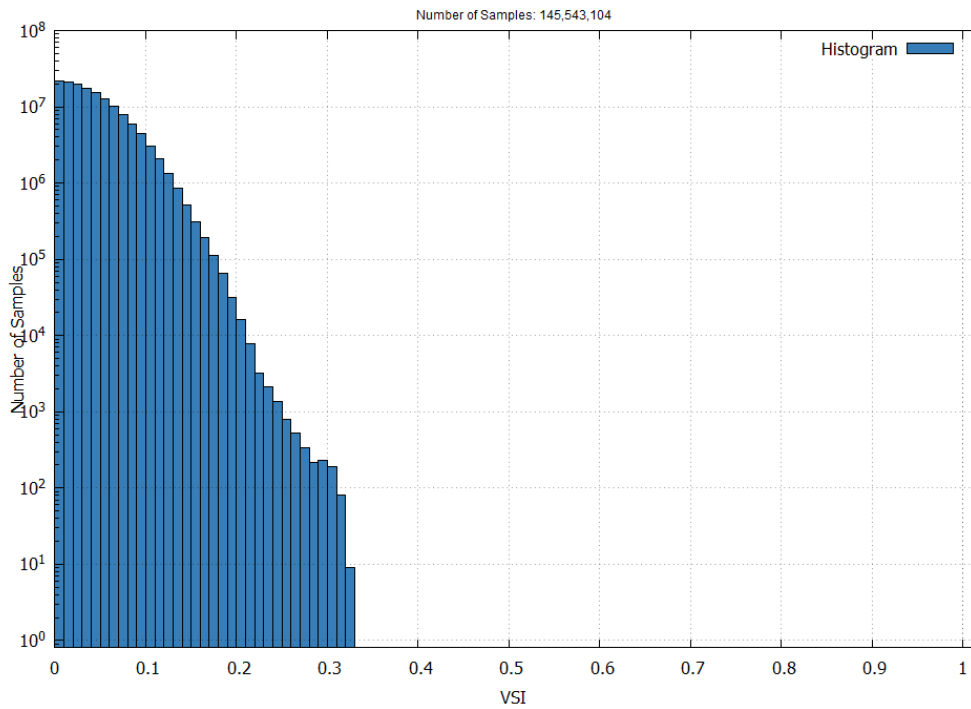
Figure 14 – EGNOS APV-I Vertical Safety Index in July 2026
