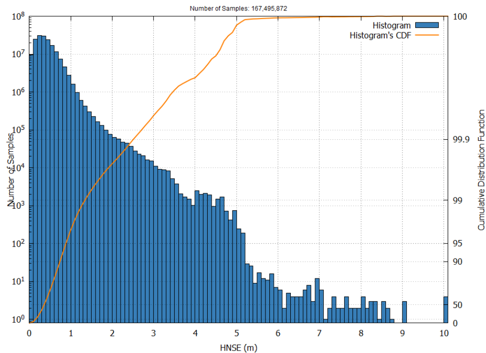
Figure 9 – EGNOS NPA HNSE Histogram and Cumulative Probability in July 2026
