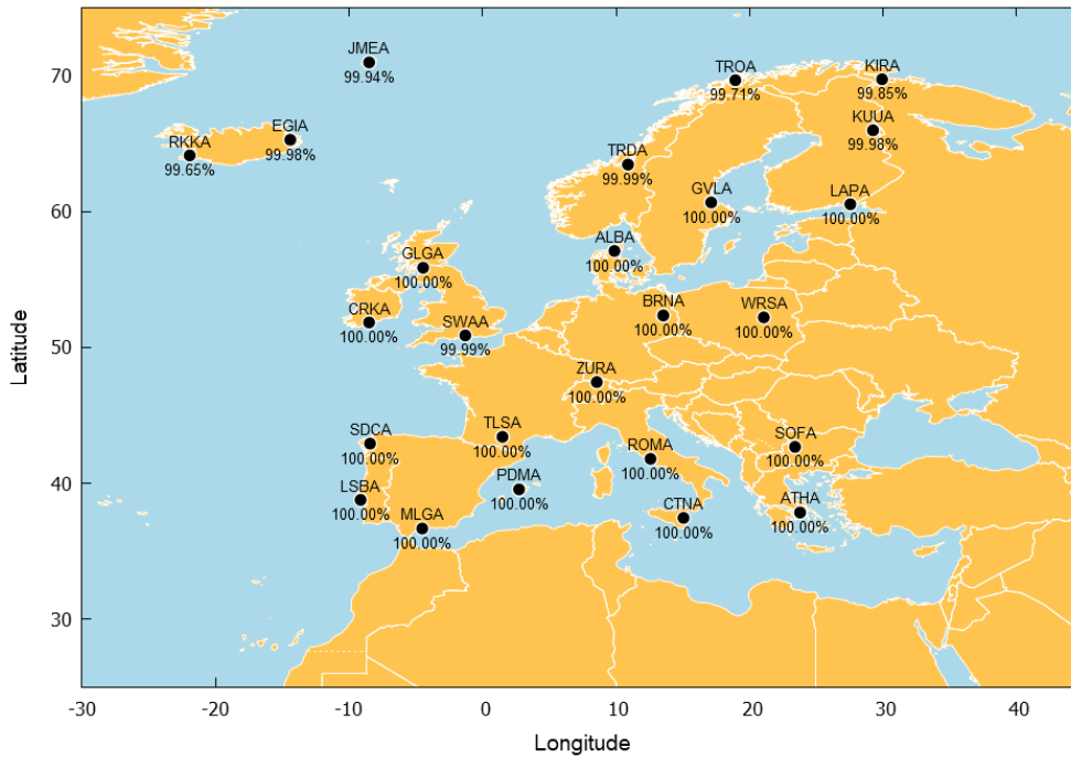
Figure 5 – EGNOS Open Service Availability at reference stations in May 2026
