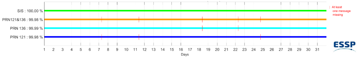
Figure 1 - EGNOS SIS & PRN Availability for May 2026
