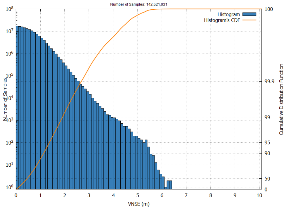
Figure 25 – EGNOS LPV-200 VNSE Histogram and Cumulative Probability in May 2026
