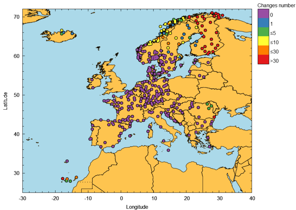
Figure 18 – EGNOS APV-I outages in May 2026
