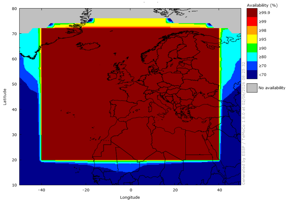
Figure 6 – EGNOS NPA Availability in May 2026
