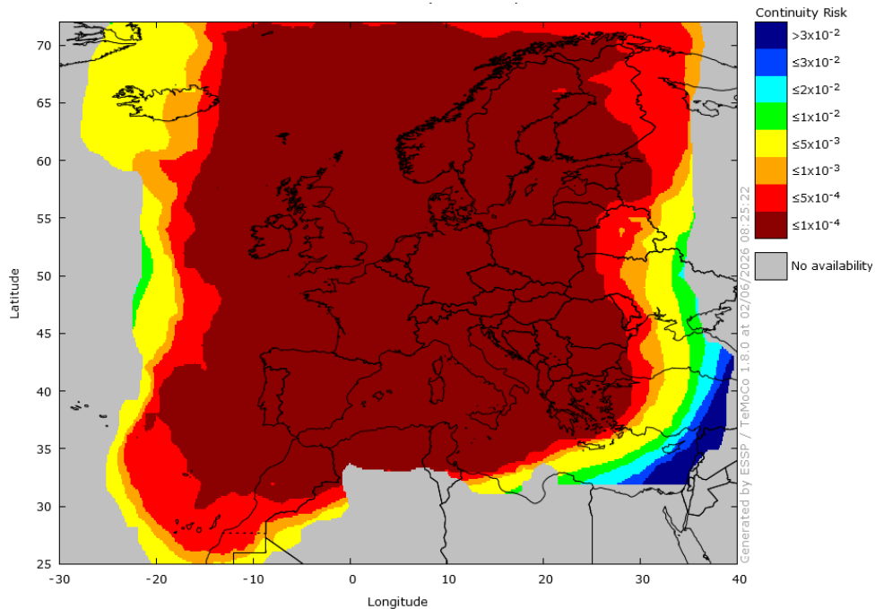
Figure 21 – EGNOS LPV-200 Continuity 2 in May 2026
