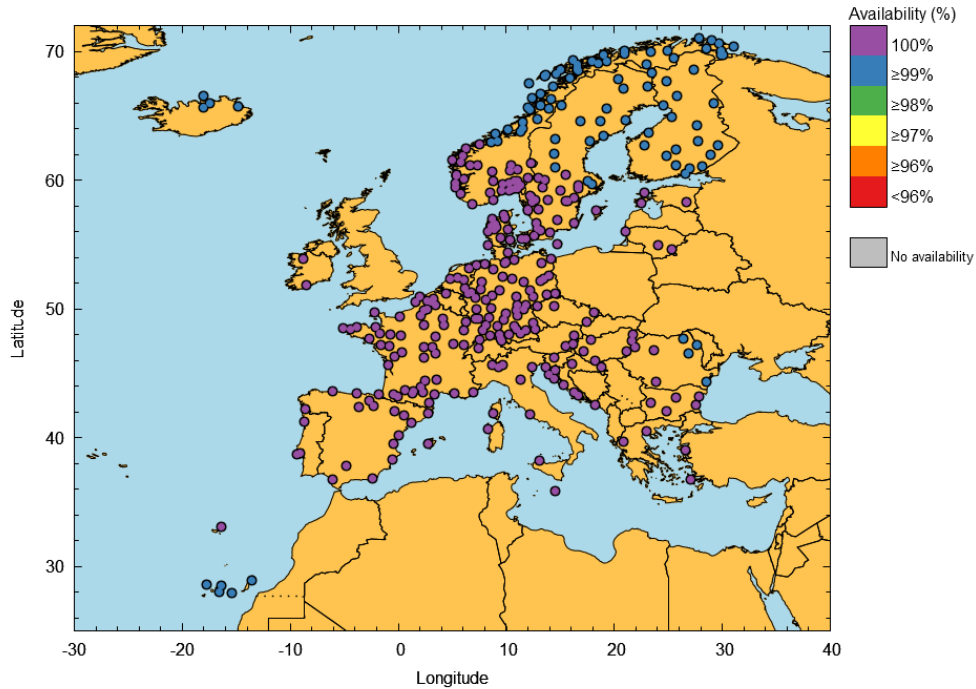
Figure 17 – EGNOS APV-I Availability at airports in May 2026
