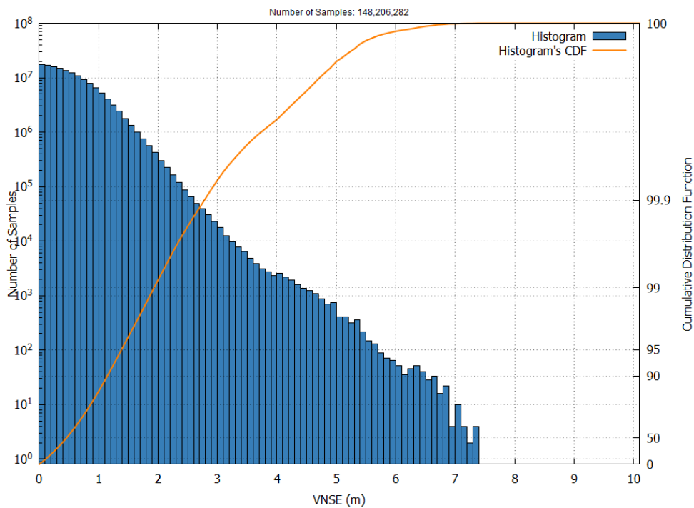
Figure 16 – EGNOS APV-I VNSE Histogram and Cumulative Probability in May 2026
