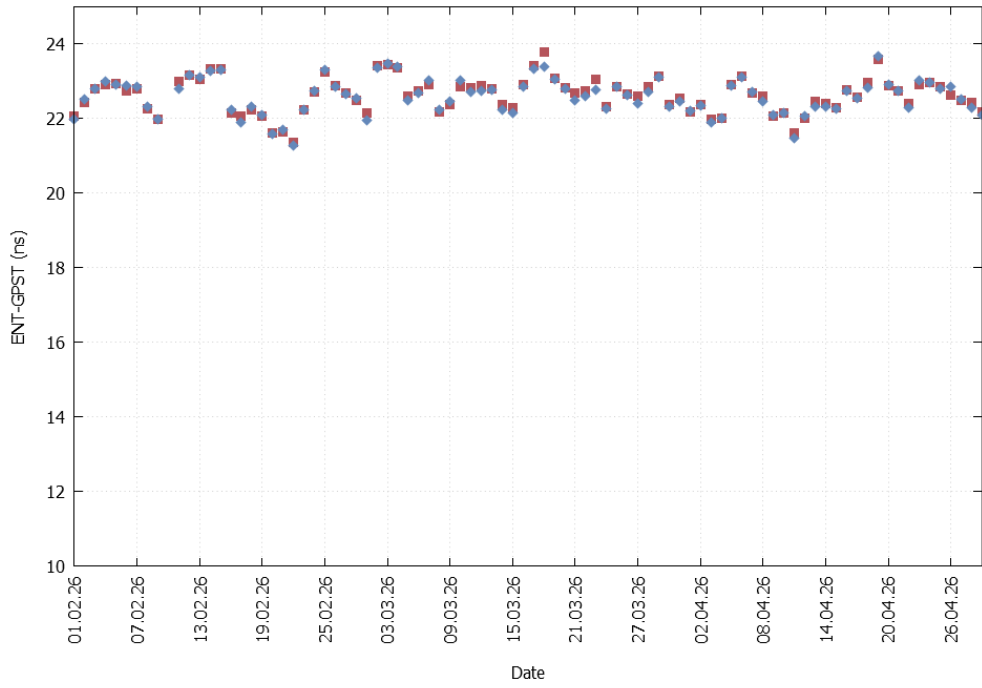
Figure 30 – ENT-GPS offset evolution from February to April 2026 (red PRN 121; blue PRN 136)
