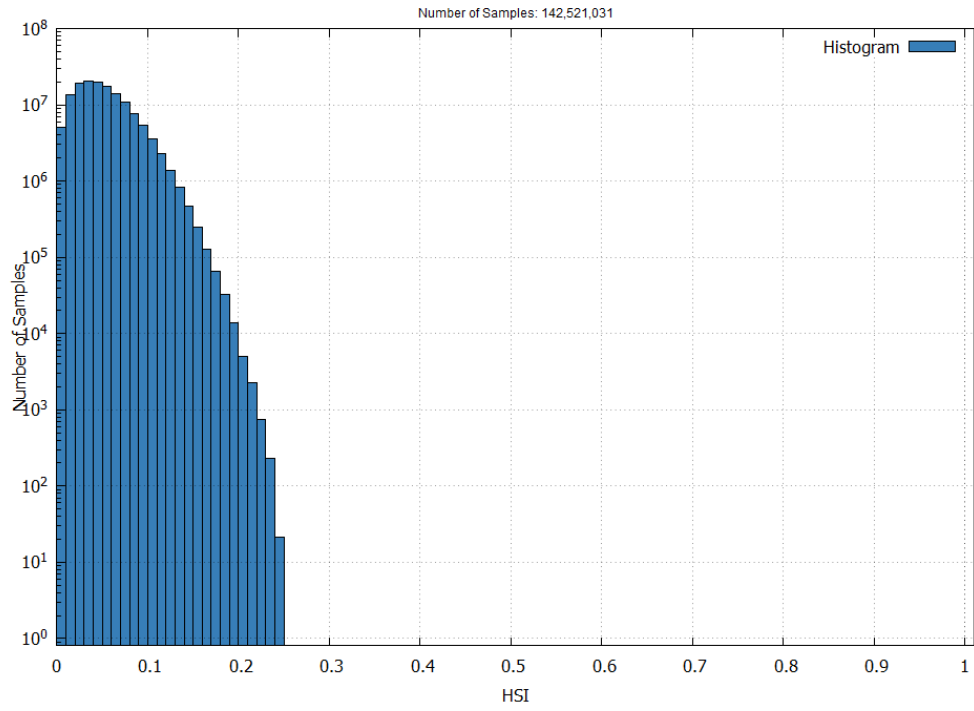
Figure 22 – EGNOS LPV-200 Horizontal Safety Index in May 2026
