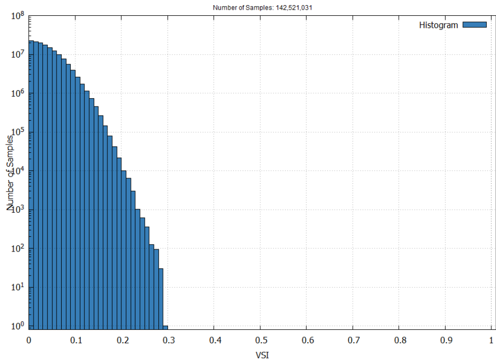
Figure 23 – EGNOS LPV-200 Vertical Safety Index in May 2026
