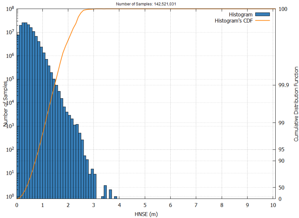
Figure 24 – EGNOS LPV-200 HNSE Histogram and Cumulative Probability in May 2026
