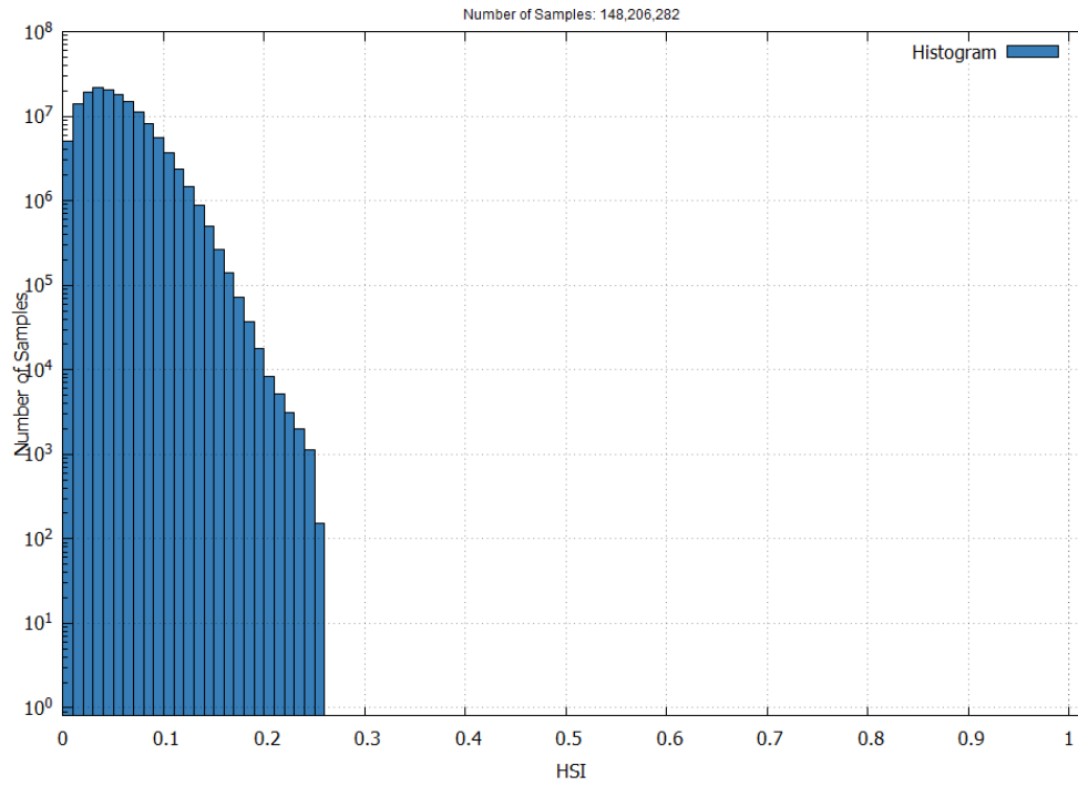
Figure 13 – EGNOS APV-I Horizontal Safety Index in May 2026
