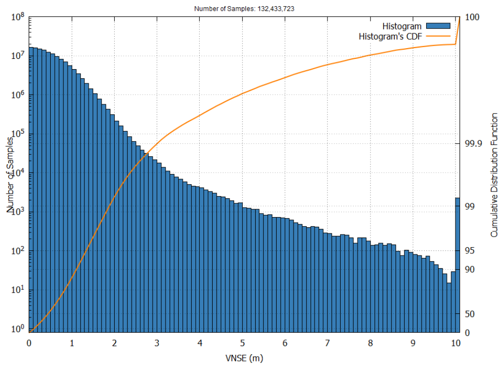
Figure 4 – EGNOS Open Service VNSE Histogram and Cumulative Probability in May 2026
