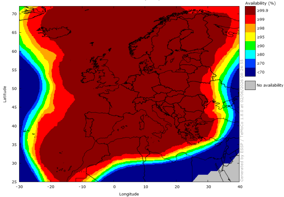
Figure 10 – EGNOS APV-I Availability in May 2026
