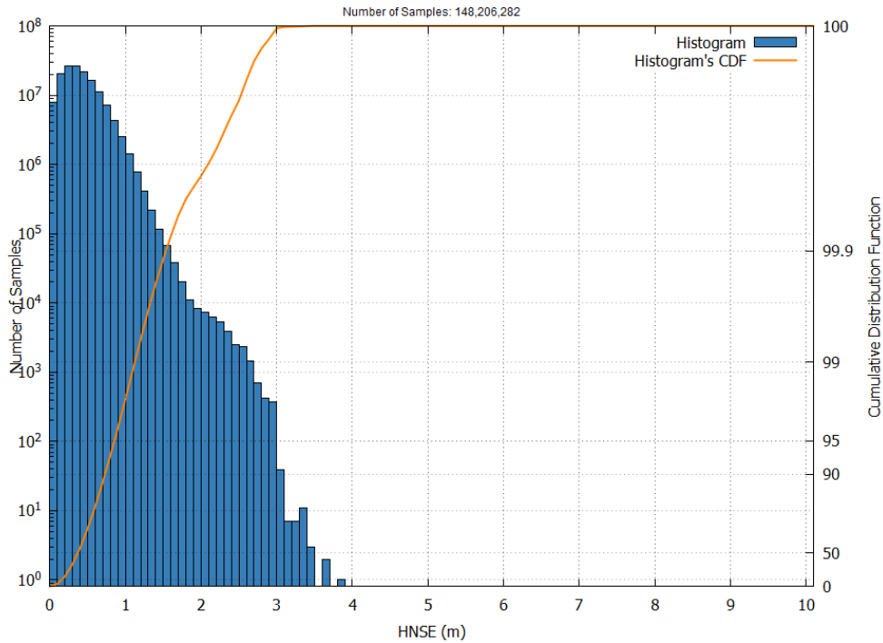
Figure 15 – EGNOS APV-I HNSE Histogram and Cumulative Probability in May 2026
