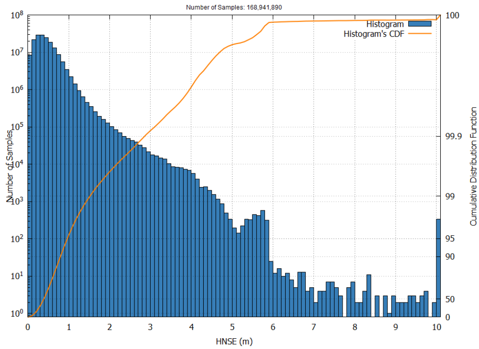
Figure 9 – EGNOS NPA HNSE Histogram and Cumulative Probability in May 2026
