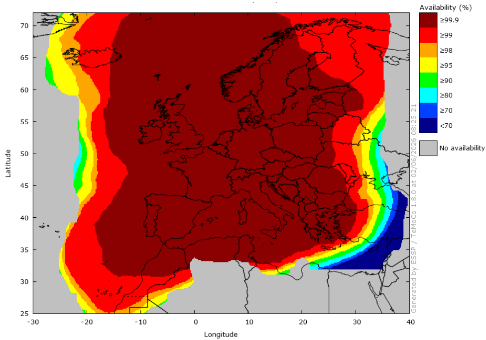
Figure 19 – EGNOS LPV-200 Availability in May 2026
