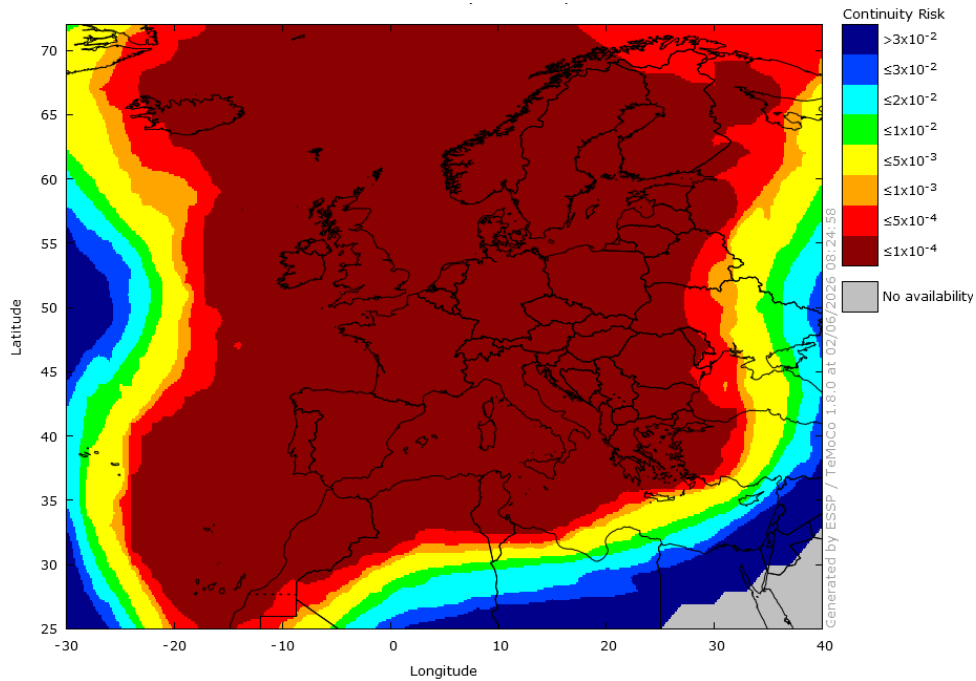
Figure 12 – EGNOS APV-I Continuity in May 2026
