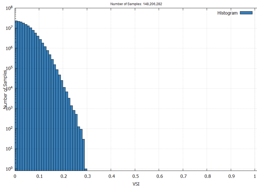
Figure 14 – EGNOS APV-I Vertical Safety Index in May 2026
