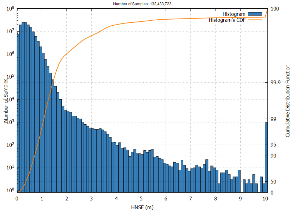
Figure 3 – EGNOS Open Service HNSE Histogram and Cumulative Probability in May 2026
