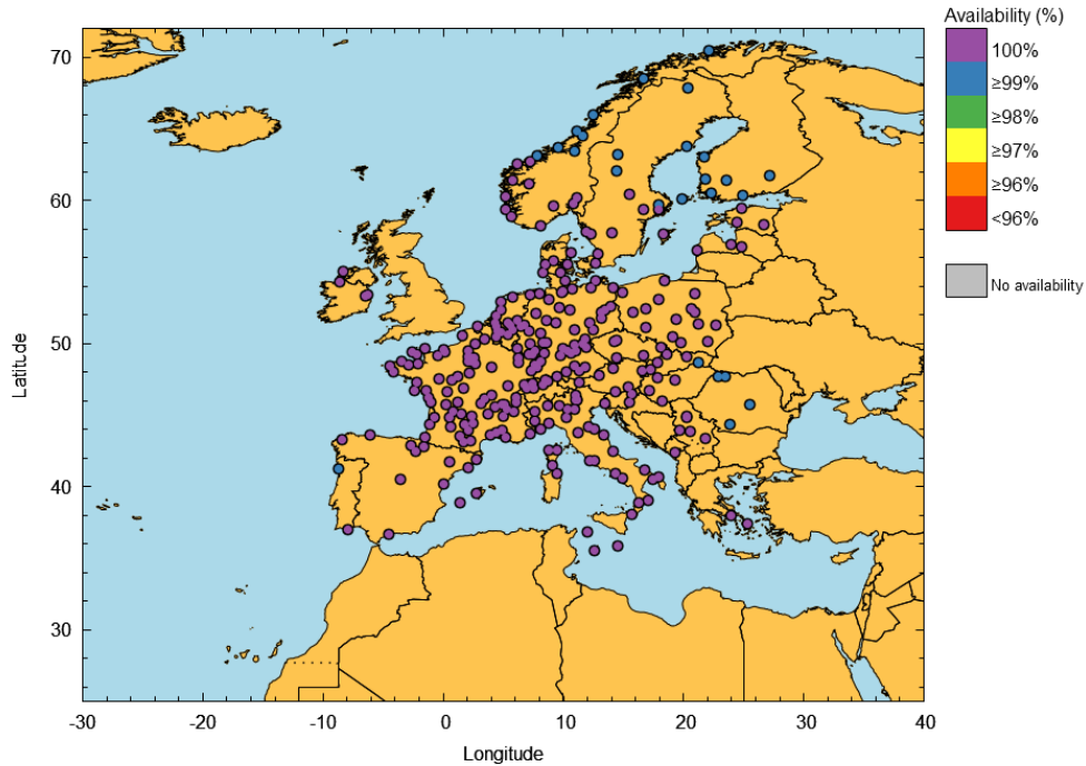
Figure 27 – EGNOS LPV-200 Availability at airports in May 2026
