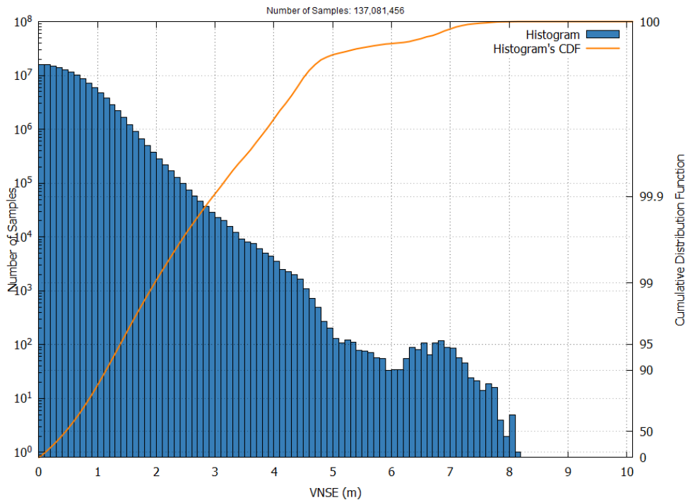
Figure 25 – EGNOS LPV-200 VNSE Histogram and Cumulative Probability in April 2026
