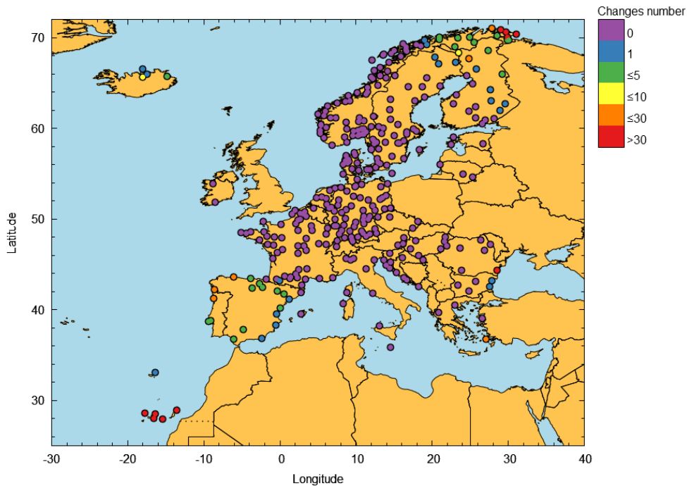
Figure 18 – EGNOS APV-I outages in April 2026
