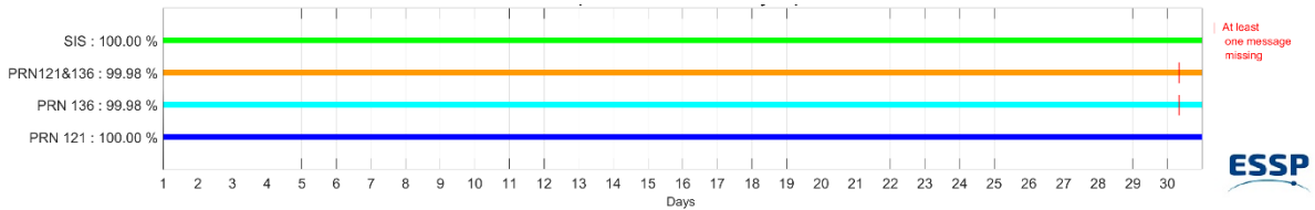
Figure 1 - EGNOS SIS & PRN Availability for April 2026
