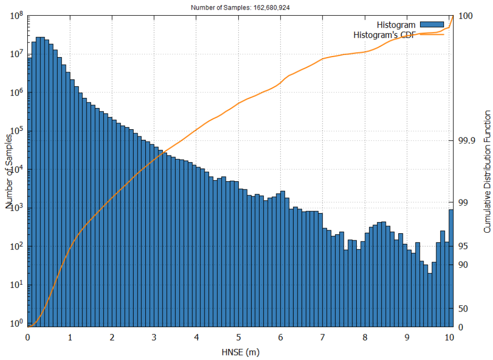
Figure 9 – EGNOS NPA HNSE Histogram and Cumulative Probability in April 2026
