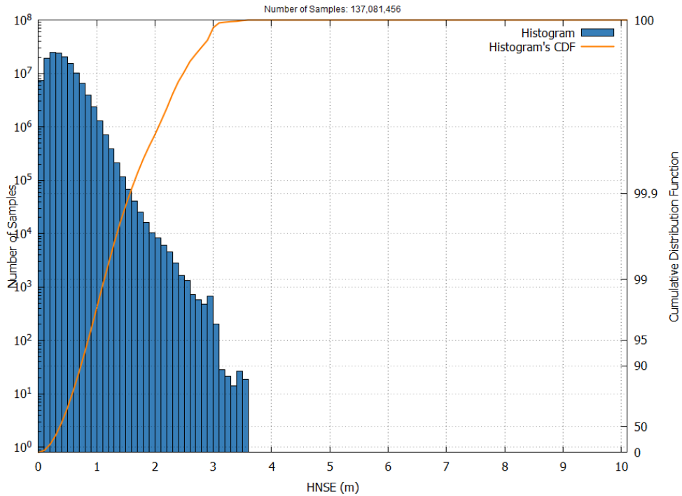
Figure 24 – EGNOS LPV-200 HNSE Histogram and Cumulative Probability in April 2026
