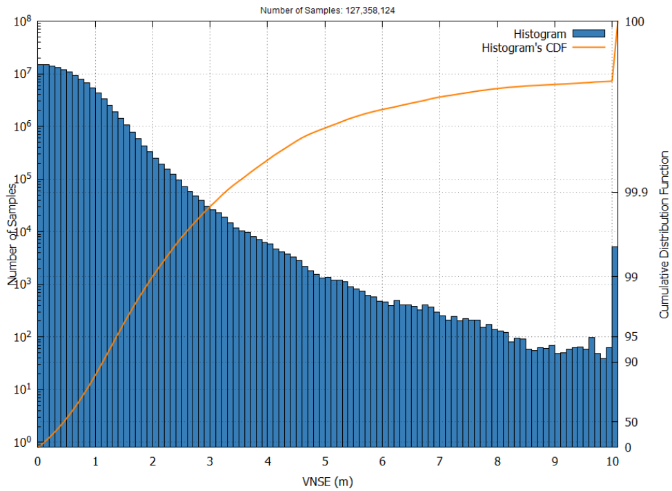
Figure 4 – EGNOS Open Service VNSE Histogram and Cumulative Probability in April 2026
