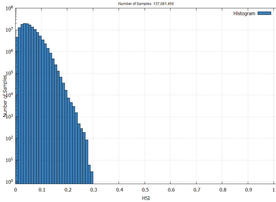
Figure 22 – EGNOS LPV-200 Horizontal Safety Index in April 2026
