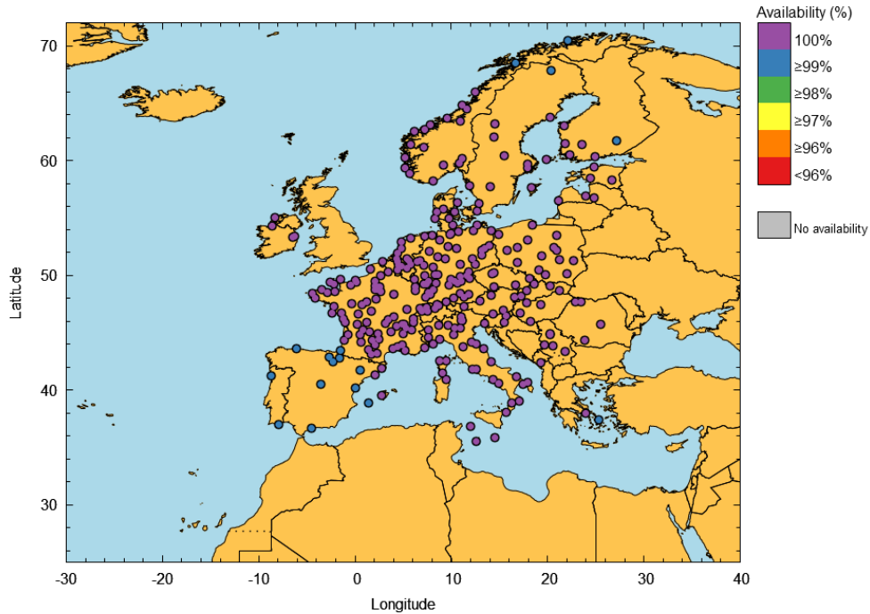
Figure 27 – EGNOS LPV-200 Availability at airports in April 2026
