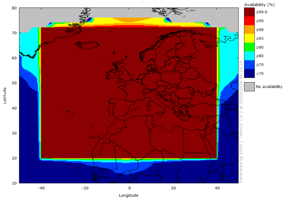
Figure 6 – EGNOS NPA Availability in April 2026
