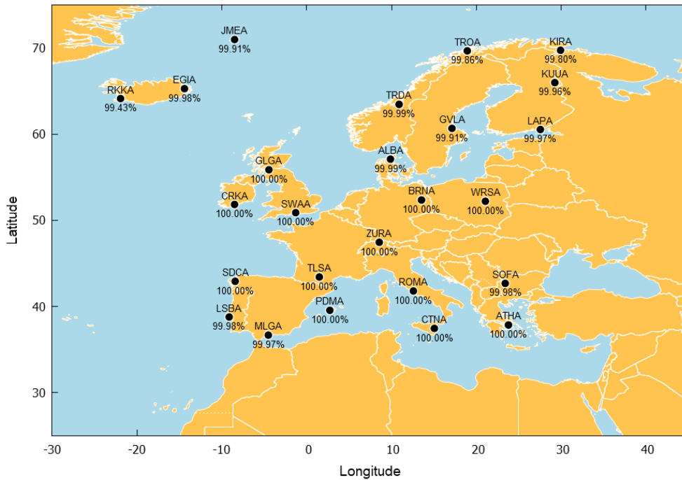
Figure 5 – EGNOS Open Service Availability at reference stations in April 2026
