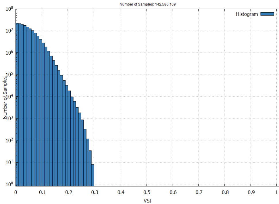
Figure 14 – EGNOS APV-I Vertical Safety Index in April 2026
