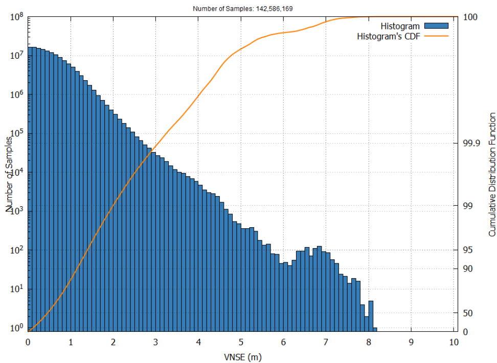
Figure 16 – EGNOS APV-I VNSE Histogram and Cumulative Probability in April 2026
