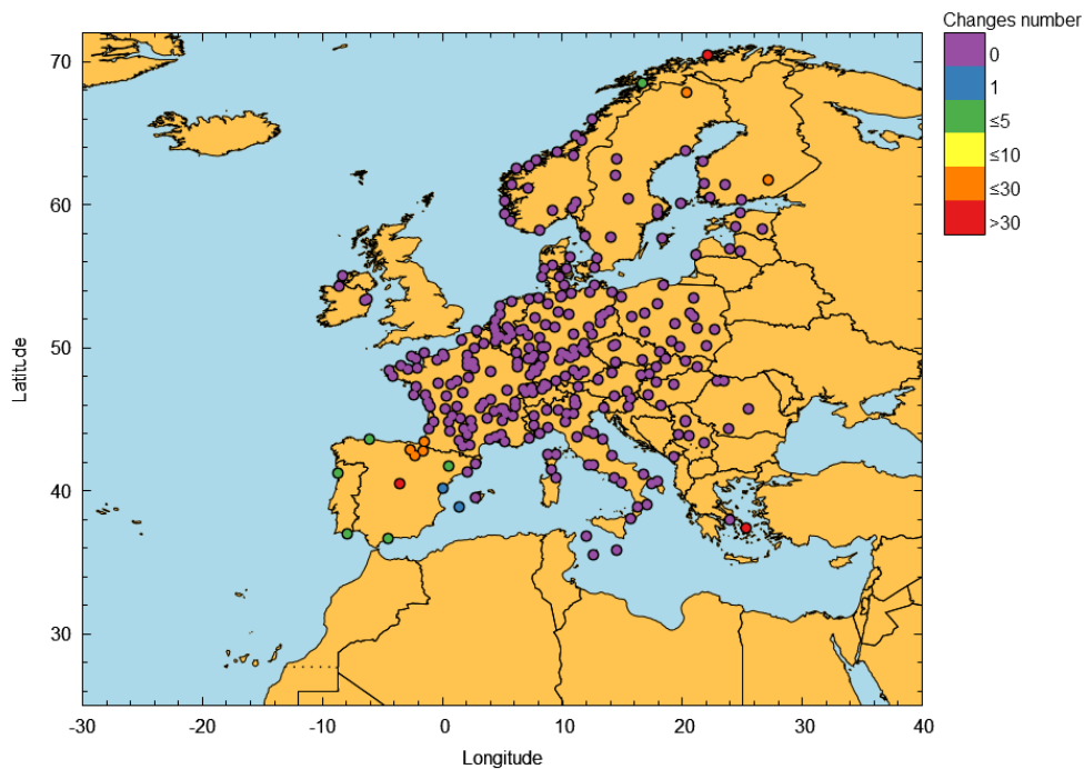
Figure 28 – EGNOS LPV-200 outages in April 2026
