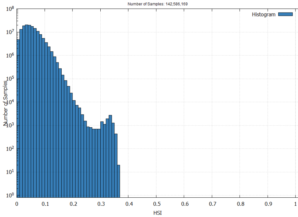
Figure 13 – EGNOS APV-I Horizontal Safety Index in April 2026
