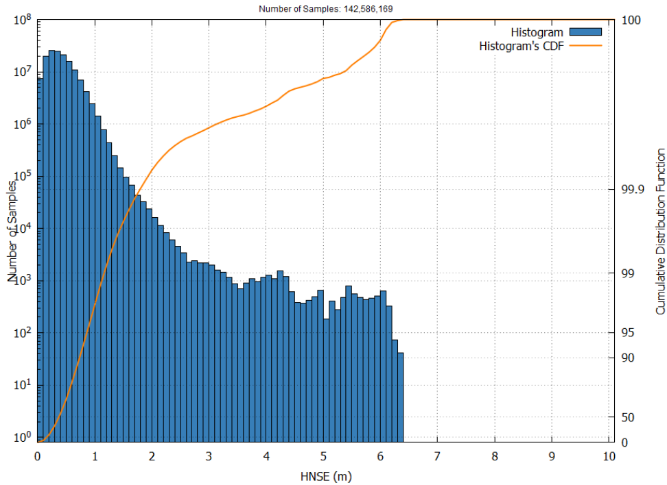
Figure 15 – EGNOS APV-I HNSE Histogram and Cumulative Probability in April 2026
