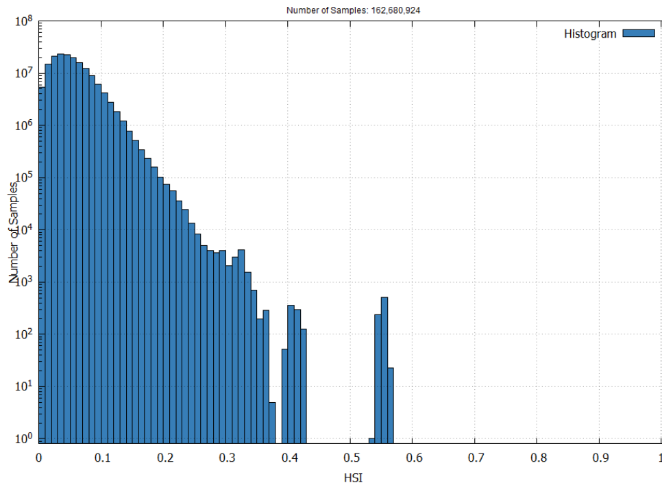
Figure 8 – EGNOS NPA Horizontal Safety Index in April 2026
