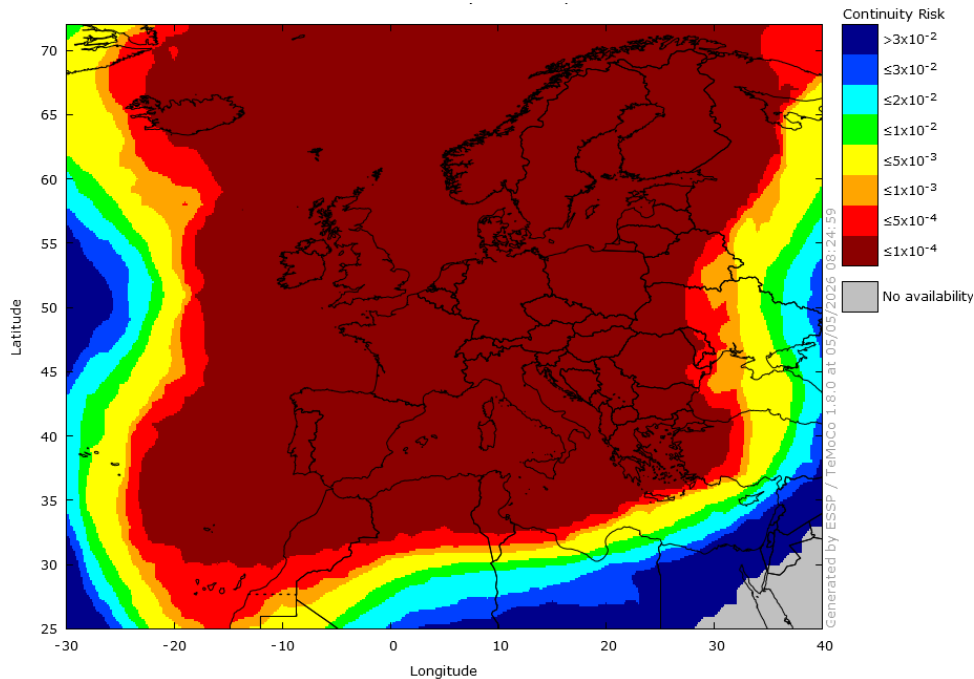
Figure 12 – EGNOS APV-I Continuity in April 2026
