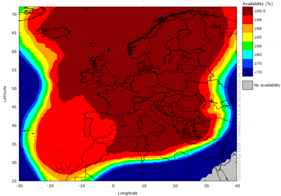
Figure 10 – EGNOS APV-I Availability in April 2026
