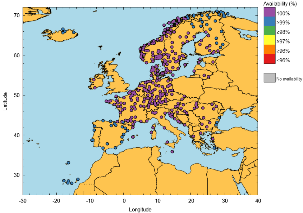
Figure 17 – EGNOS APV-I Availability at airports in April 2026
