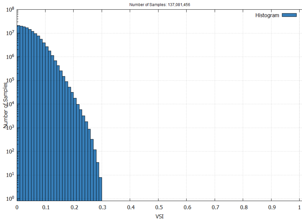
Figure 23 – EGNOS LPV-200 Vertical Safety Index in April 2026
