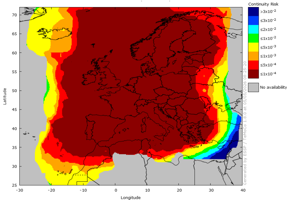
Figure 21 – EGNOS LPV-200 Continuity 2 in April 2026
