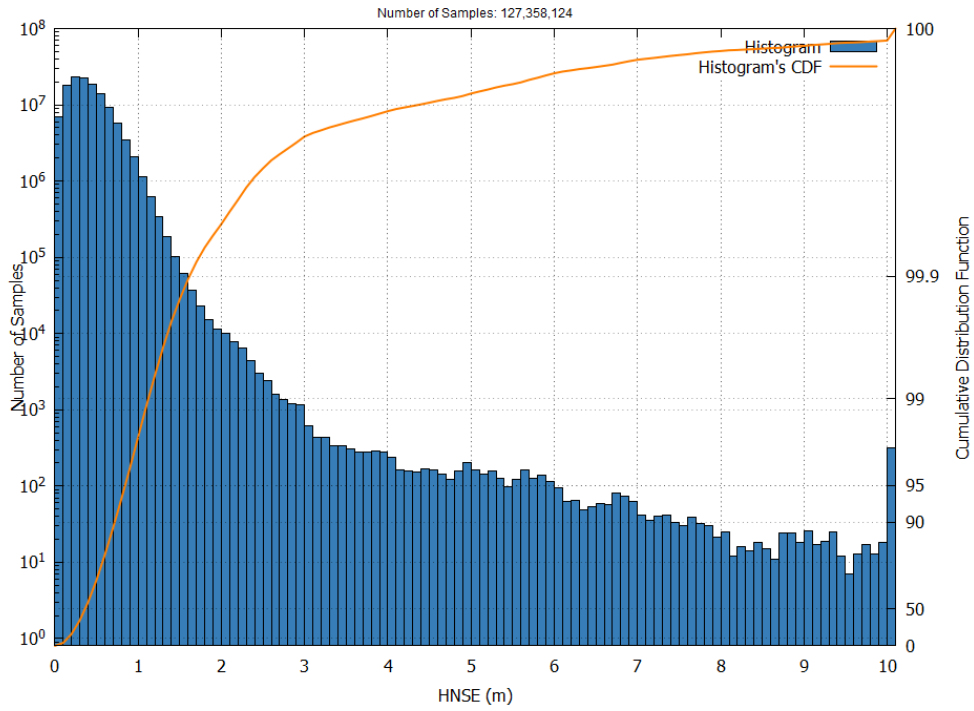
Figure 3 – EGNOS Open Service HNSE Histogram and Cumulative Probability in April 2026
