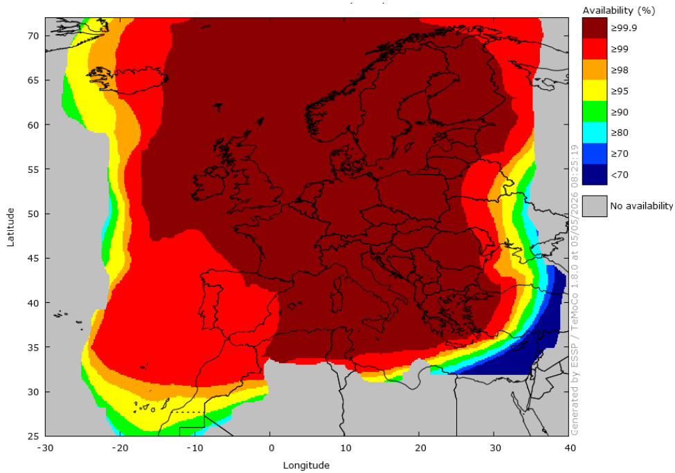
Figure 19 – EGNOS LPV-200 Availability in April 2026
