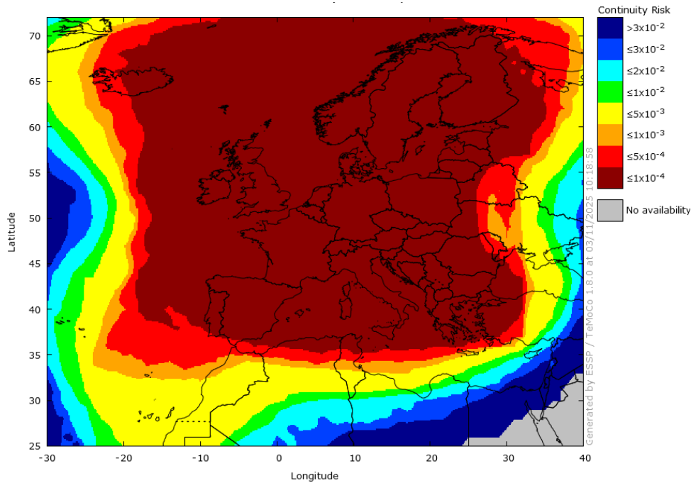
Figure 12 – EGNOS APV-I Continuity in October 2025 (Excluding data from the 13th to the 17th of October)
