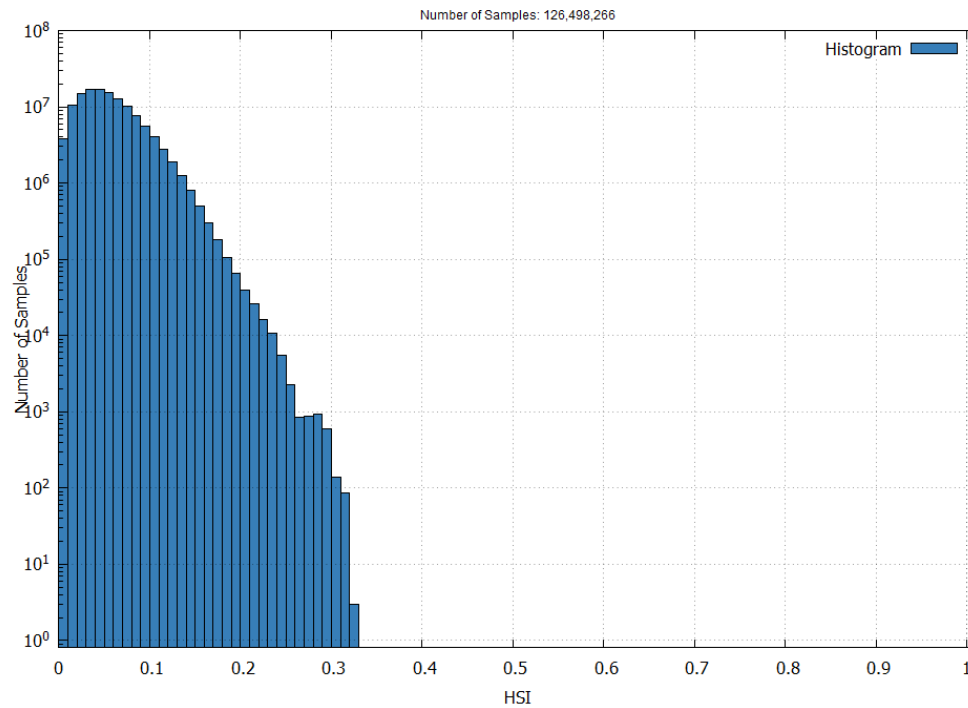
Figure 13 – EGNOS APV-I Horizontal Safety Index in October 2025 (Excluding data from the 13th to the 17th of October)
