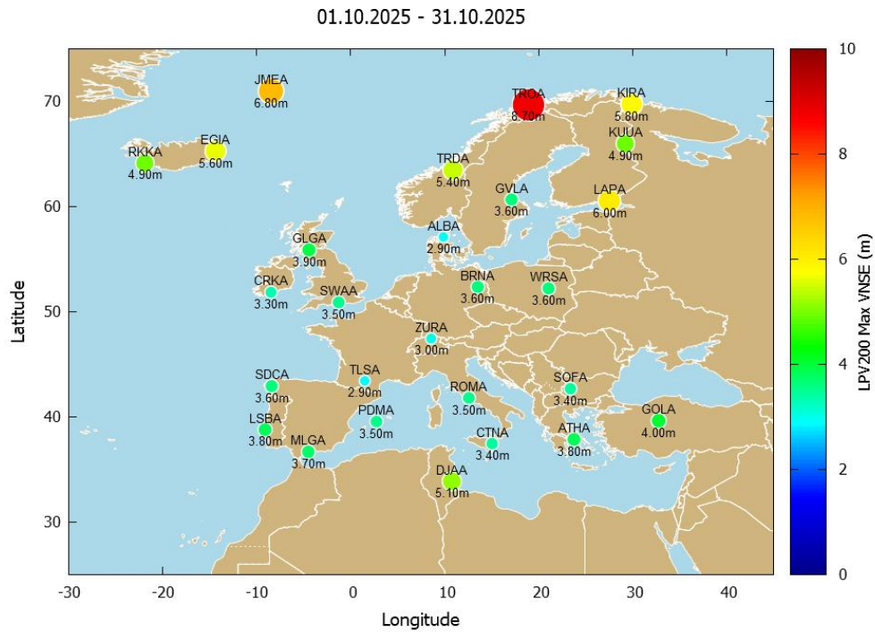
Figure 26 – EGNOS LPV-200 VNSE Maximum Values (Excluding data from the 13th to the 17th of October)
