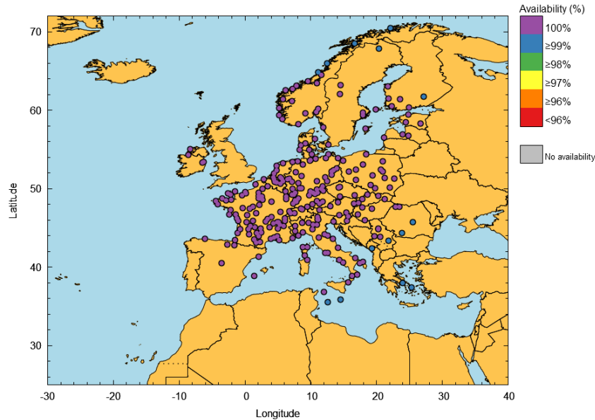
Figure 27 – EGNOS LPV-200 Availability at airports in October 2025 (Excluding data from the 13th to the 17th of October)
