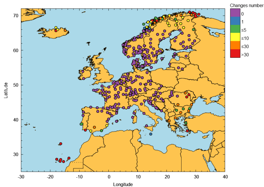
Figure 18 – EGNOS APV-I outages in October 2025 (Excluding data from the 13th to the 17th of October)
