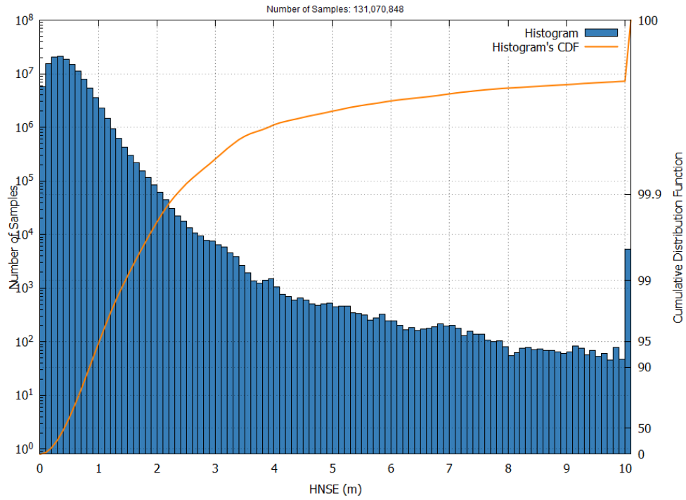
Figure 3 – EGNOS Open Service HNSE Histogram and Cumulative Probability in October 2025
