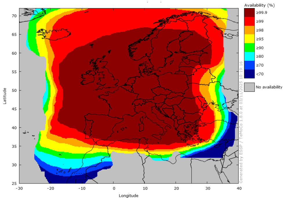
Figure 19 – EGNOS LPV-200 Availability in October 2025 (Excluding data from the 13th to the 17th of October)
