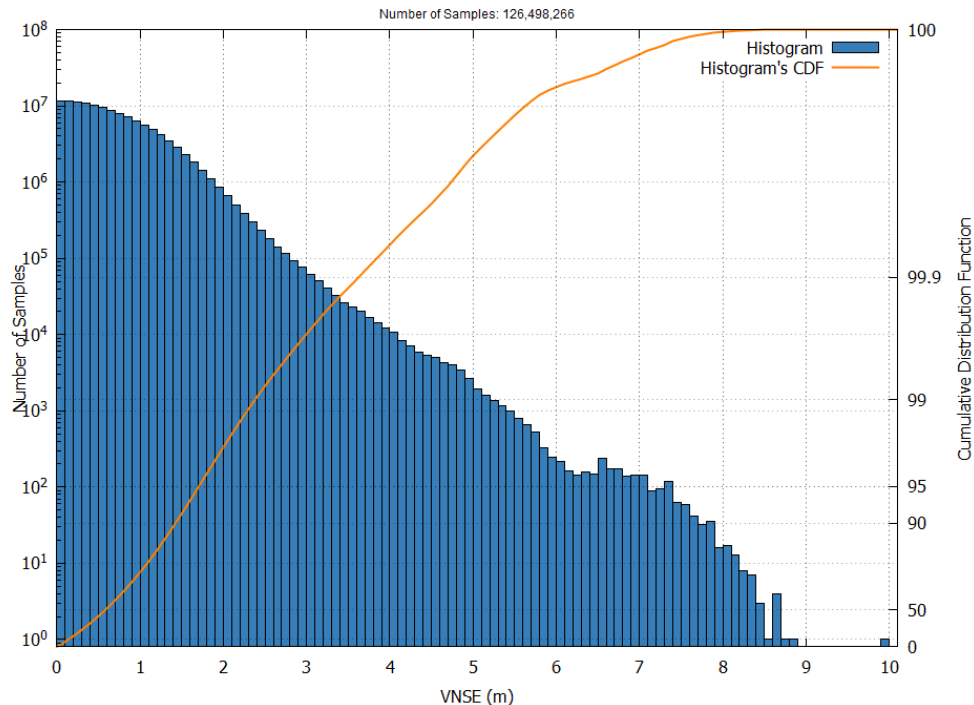
Figure 16 – EGNOS APV-I VNSE Histogram and Cumulative Probability in October 2025 (Excluding data from the 13th to the 17th of October)
