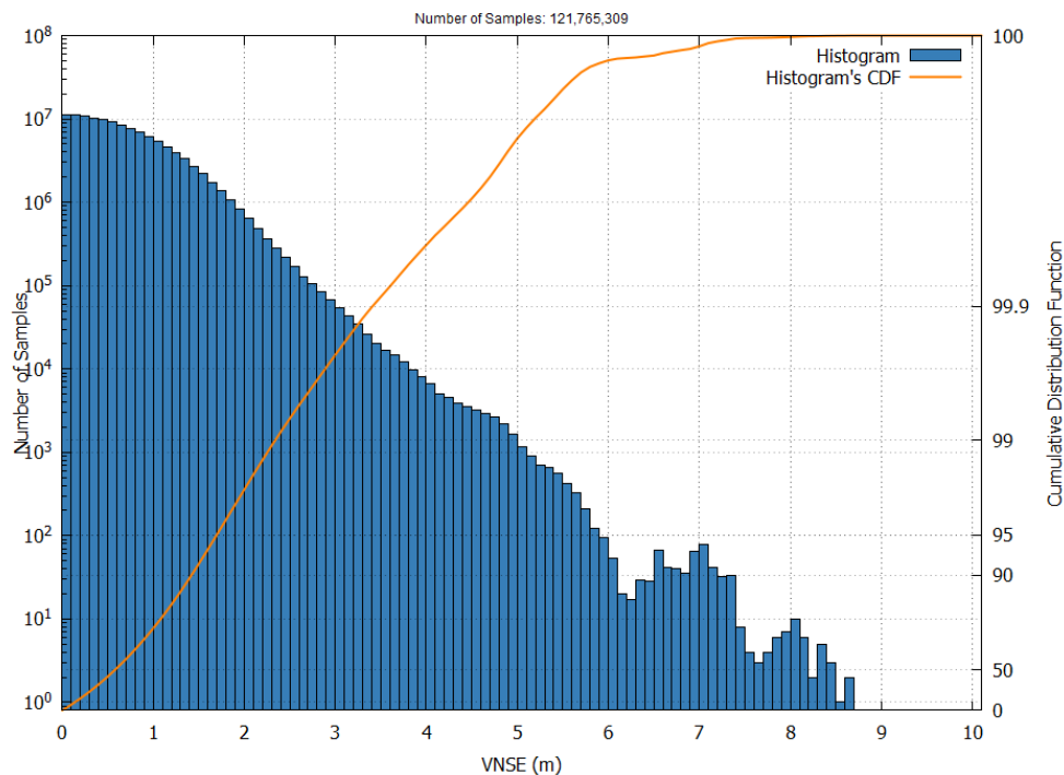
Figure 25 – EGNOS LPV-200 VNSE Histogram and Cumulative Probability in October 2025 (Excluding data from the 13th to the 17th of October)
