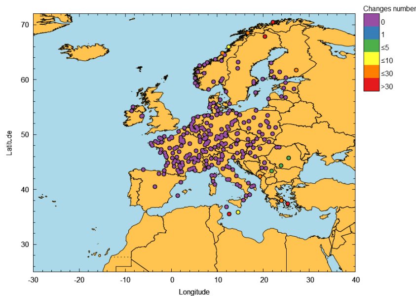
Figure 28 – EGNOS LPV-200 outages in October 2025 (Excluding data from the 13th to the 17th of October)
