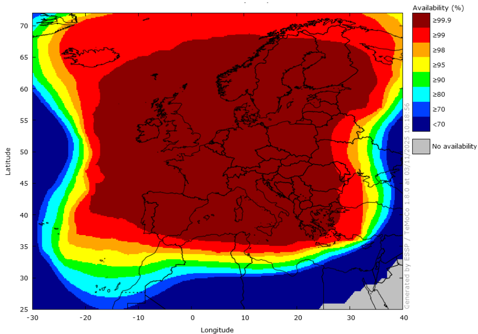
Figure 10 – EGNOS APV-I Availability in October 2025 (Excluding data from the 13th to the 17th of October)
