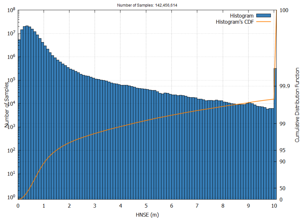
Figure 9 – EGNOS NPA HNSE Histogram and Cumulative Probability in October 2025 (Excluding data from the 13th to the 17th of October)
