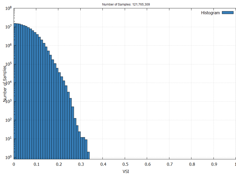
Figure 23 – EGNOS LPV-200 Vertical Safety Index in October 2025 (Excluding data from the 13th to the 17th of October)
