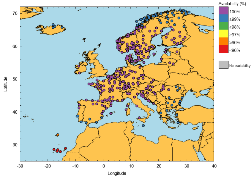
Figure 17 – EGNOS APV-I Availability at airports in October 2025 (Excluding data from the 13th to the 17th of October)
