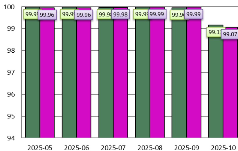
Figure 2 – Trend of EGNOS SIS Availability per GEO for the past 6 (in green PRN 136; in purple PRN 121 until 8th September and PRN 121 from September 9th)
