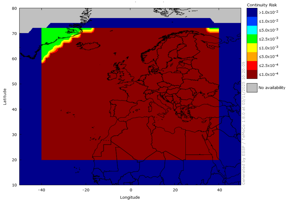
Figure 7 – EGNOS NPA Continuity over the last 6 months (Excluding data from the 13th to the 17th of October)
