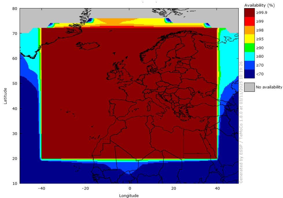
Figure 6 – EGNOS NPA Availability in October 2025 (Excluding data from the 13th to the 17th of October)
