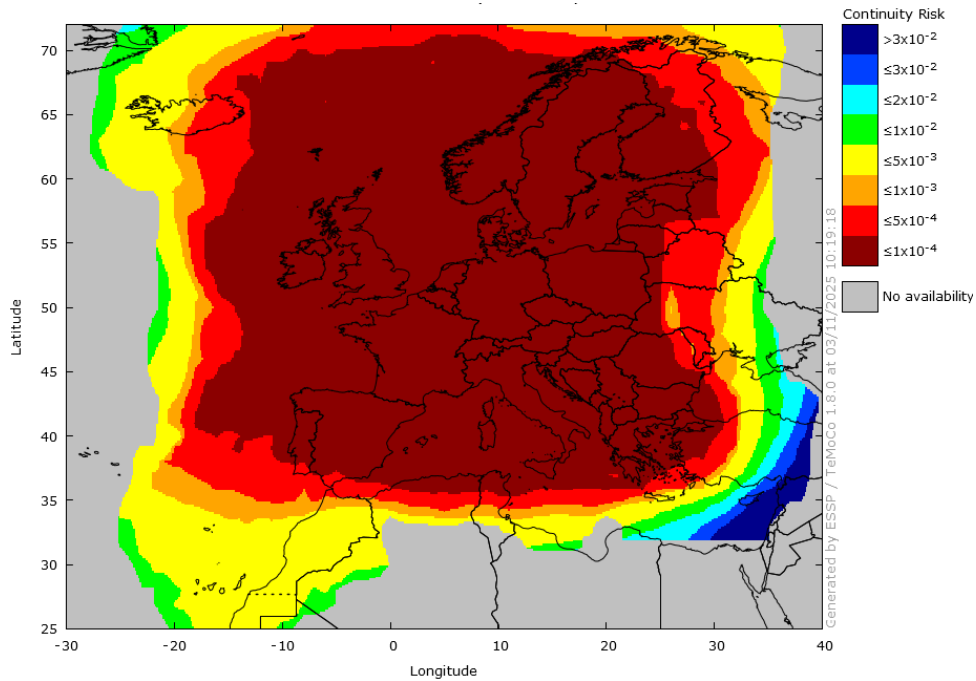
Figure 21 – EGNOS LPV-200 Continuity 4 in October 2025 (Excluding data from the 13th to the 17th of October)
