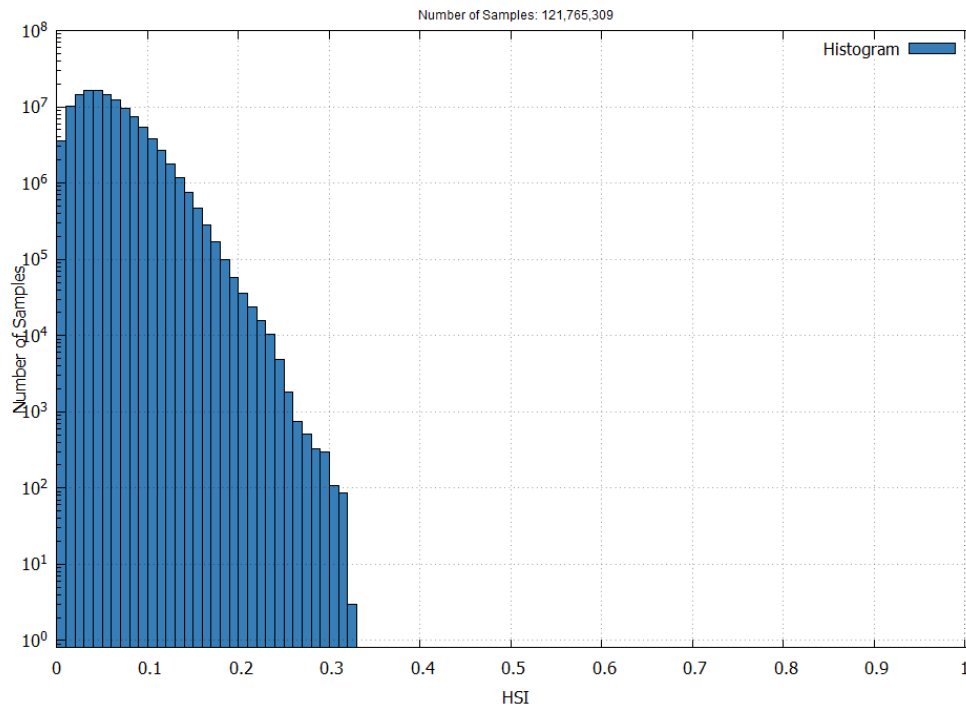
Figure 22 – EGNOS LPV-200 Horizontal Safety Index in October 2025 (Excluding data from the 13th to the 17th of October)
