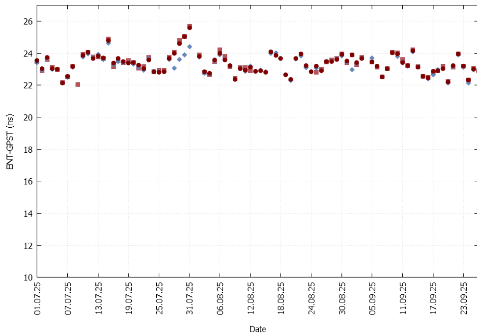
Figure 30 – ENT-GPS offset evolution from July to September 2025 (red square PRN 121; red circle PRN136; blue PRN 123)
