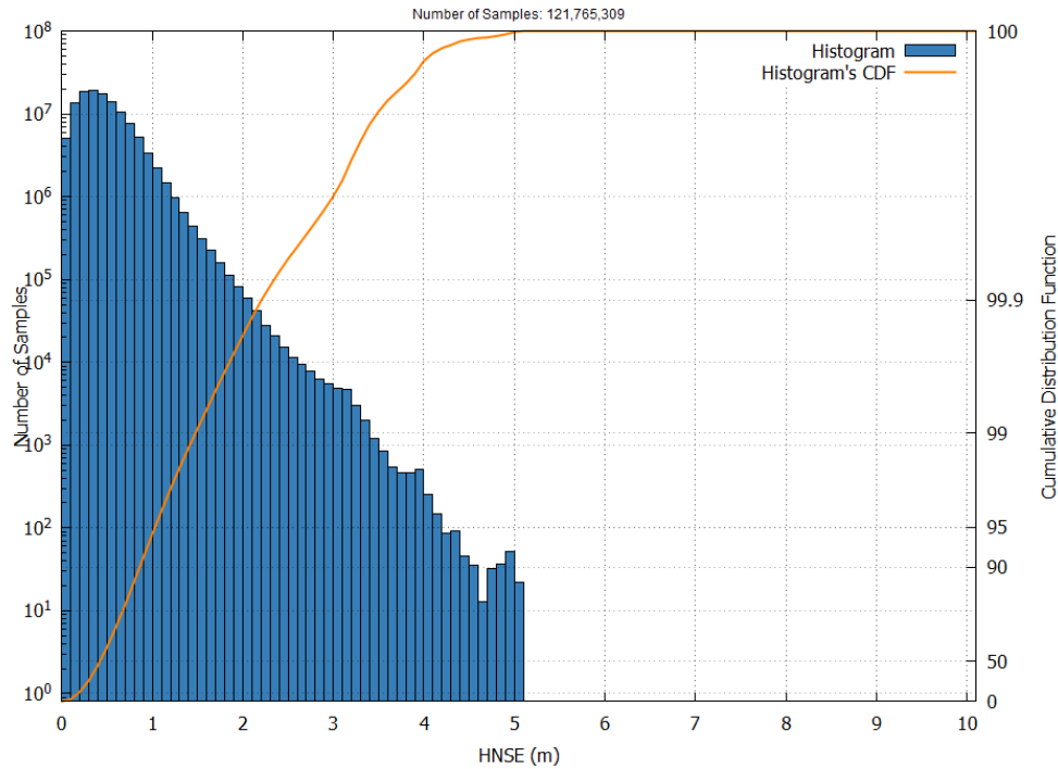
Figure 24 – EGNOS LPV-200 HNSE Histogram and Cumulative Probability in October 2025 (Excluding data from the 13th to the 17th of October)
