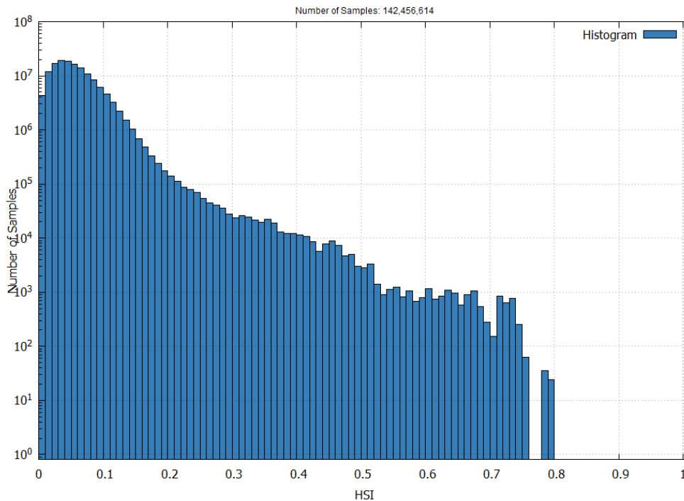
Figure 8 – EGNOS NPA Horizontal Safety Index in October 2025 (Excluding data from the 13th to the 17th of October)
