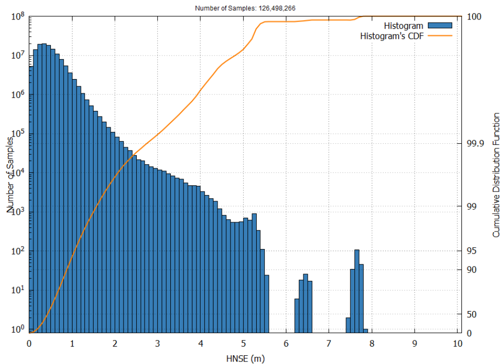
Figure 15 – EGNOS APV-I HNSE Histogram and Cumulative Probability in October 2025 (Excluding data from the 13th to the 17th of October)
