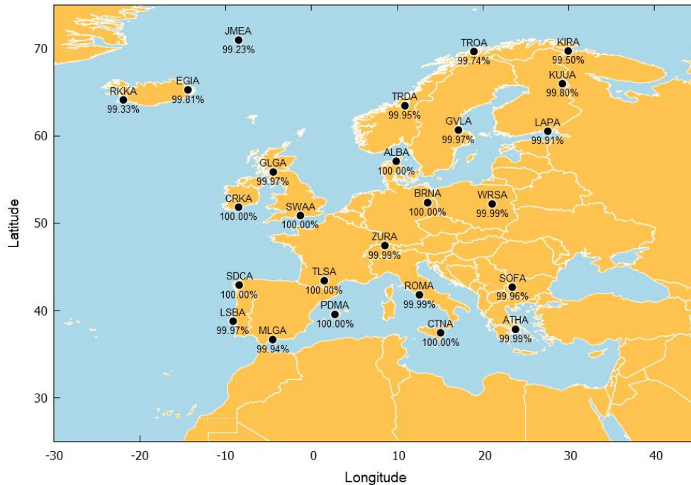
Figure 5 – EGNOS Open Service Availability at reference stations in October 2025
