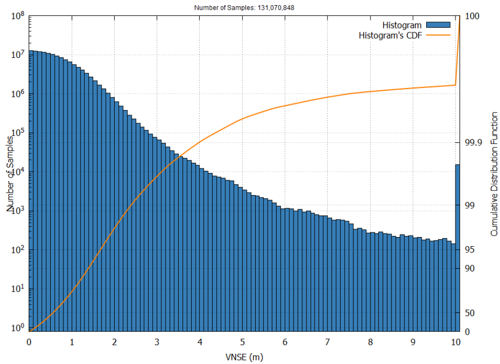
Figure 4 – EGNOS Open Service VNSE Histogram and Cumulative Probability in October 2025
