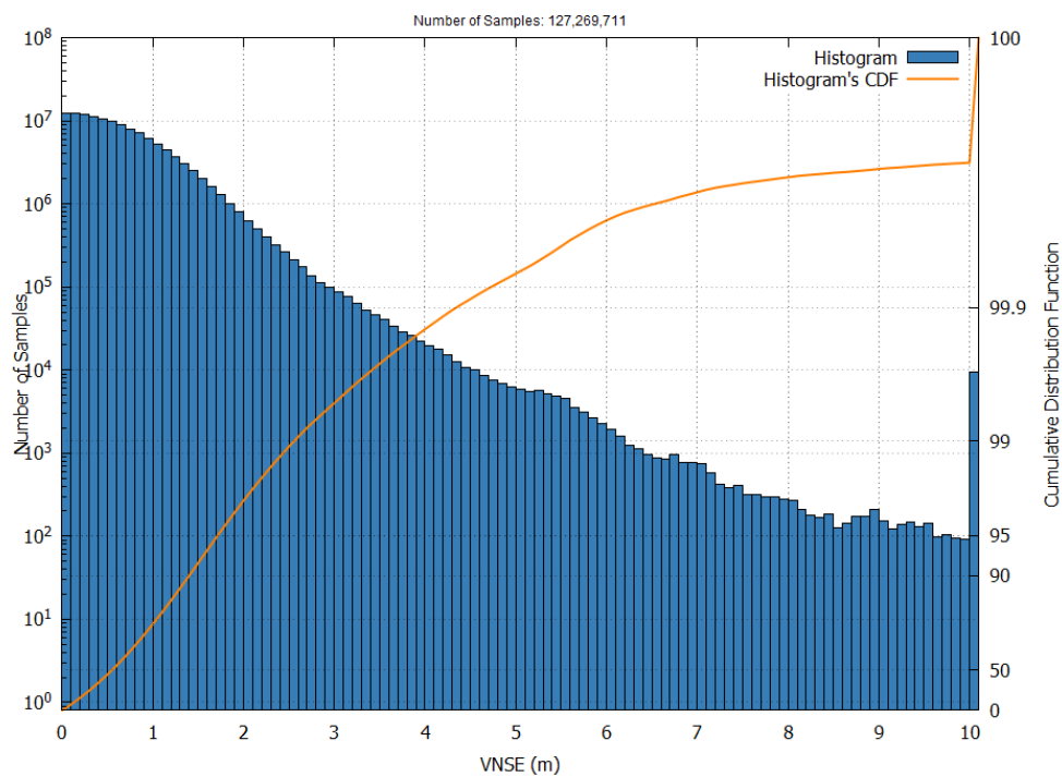
Figure 4 – EGNOS Open Service VNSE Histogram and Cumulative Probability in September 2025
