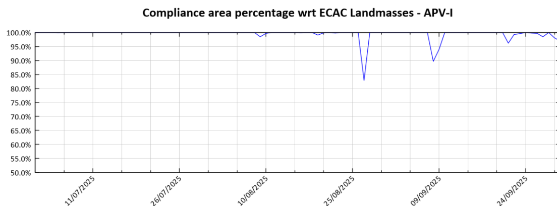
Figure 11 – EGNOS APV-I Availability compliance trend (compliance area percentage with regards to ECAC landmasses)
