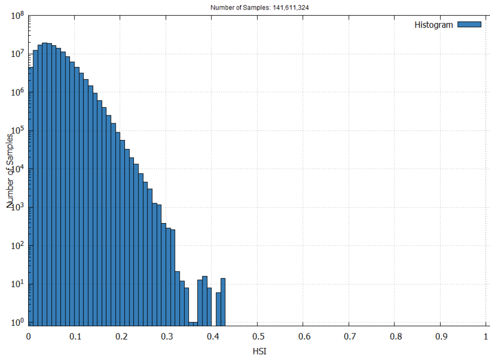
Figure 13 – EGNOS APV-I Horizontal Safety Index in September 2025
