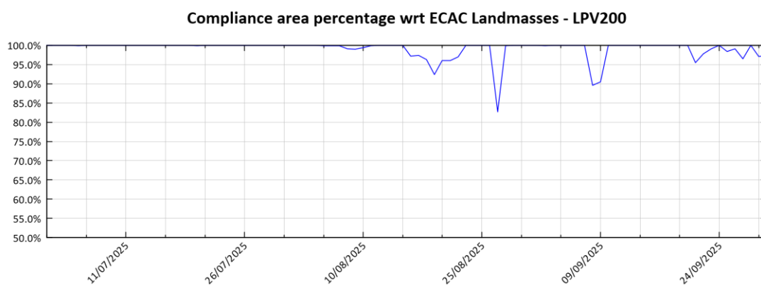
Figure 20 – EGNOS LPV-200 Availability compliance trend (compliance area percentage with regards to ECAC landmasses)
