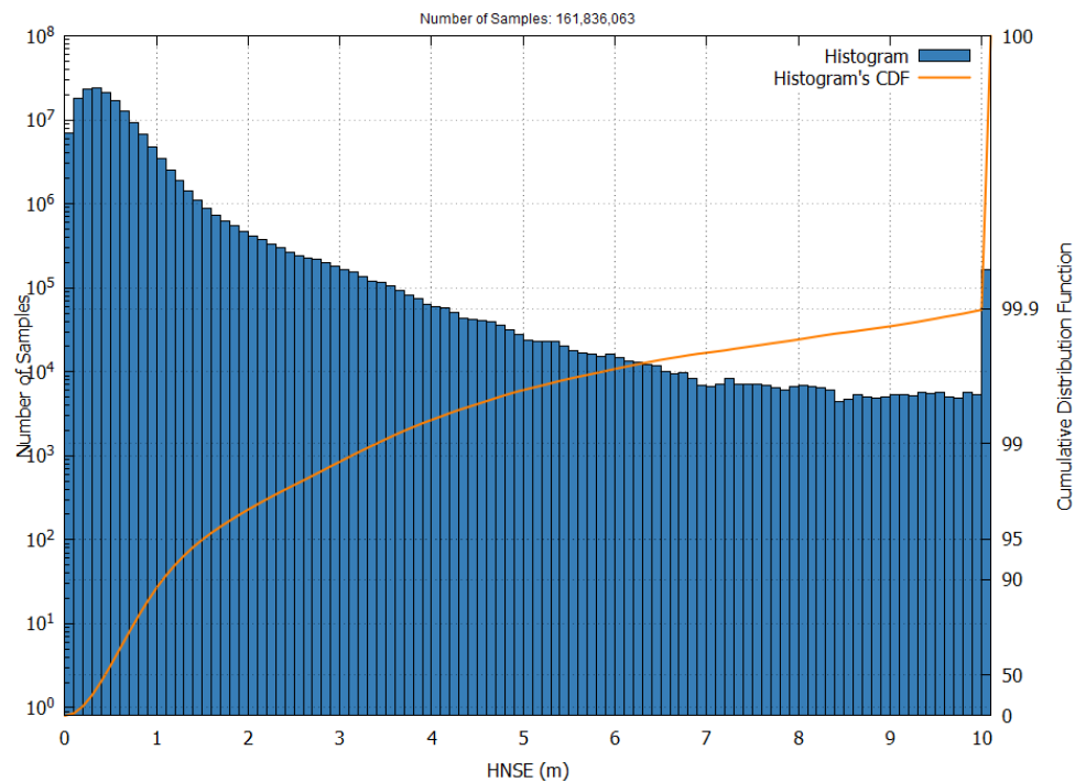
Figure 9 – EGNOS NPA HNSE Histogram and Cumulative Probability in September 2025
