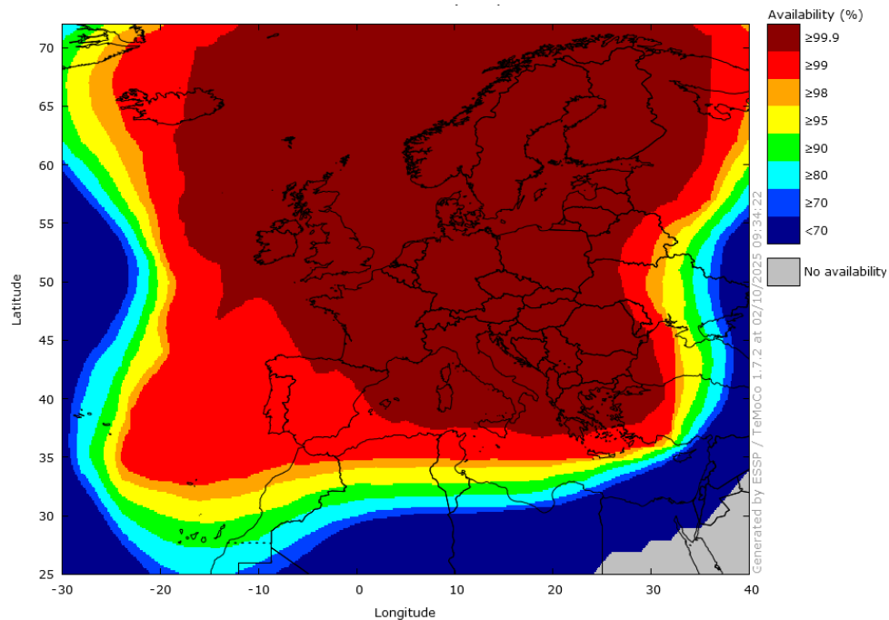
Figure 10 – EGNOS APV-I Availability in September 2025
