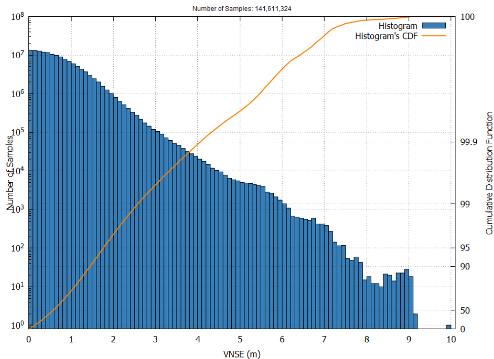
Figure 16 – EGNOS APV-I VNSE Histogram and Cumulative Probability in September 2025
