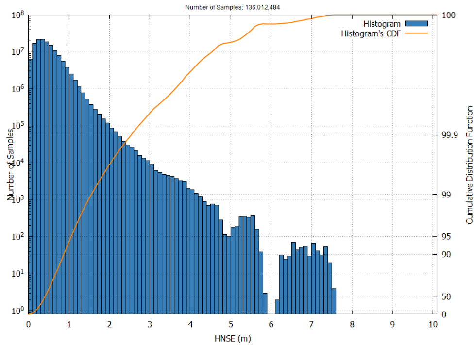
Figure 24 – EGNOS LPV-200 HNSE Histogram and Cumulative Probability in September 2025
