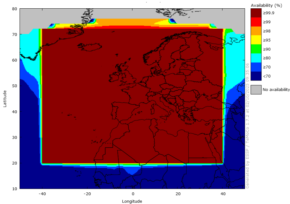
Figure 6 – EGNOS NPA Availability in September 2025
