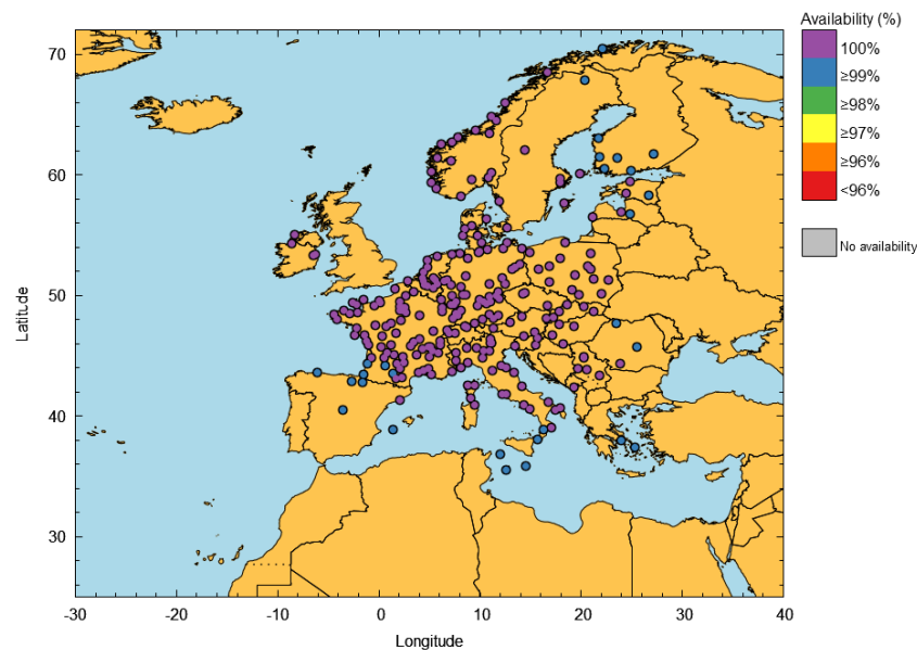
Figure 27 – EGNOS LPV-200 Availability at airports in September 2025
