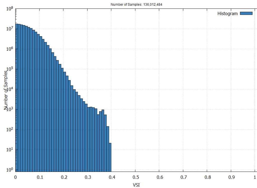
Figure 23 – EGNOS LPV-200 Vertical Safety Index in September 2025
