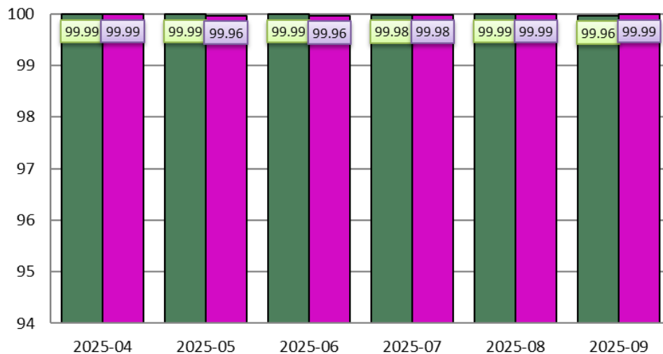
Figure 2 – Trend of EGNOS SIS Availability per GEO for the past 6 months (in green PRN 136; in purple PRN 123 until 8 th September and PRN 121 from September 9 th )
