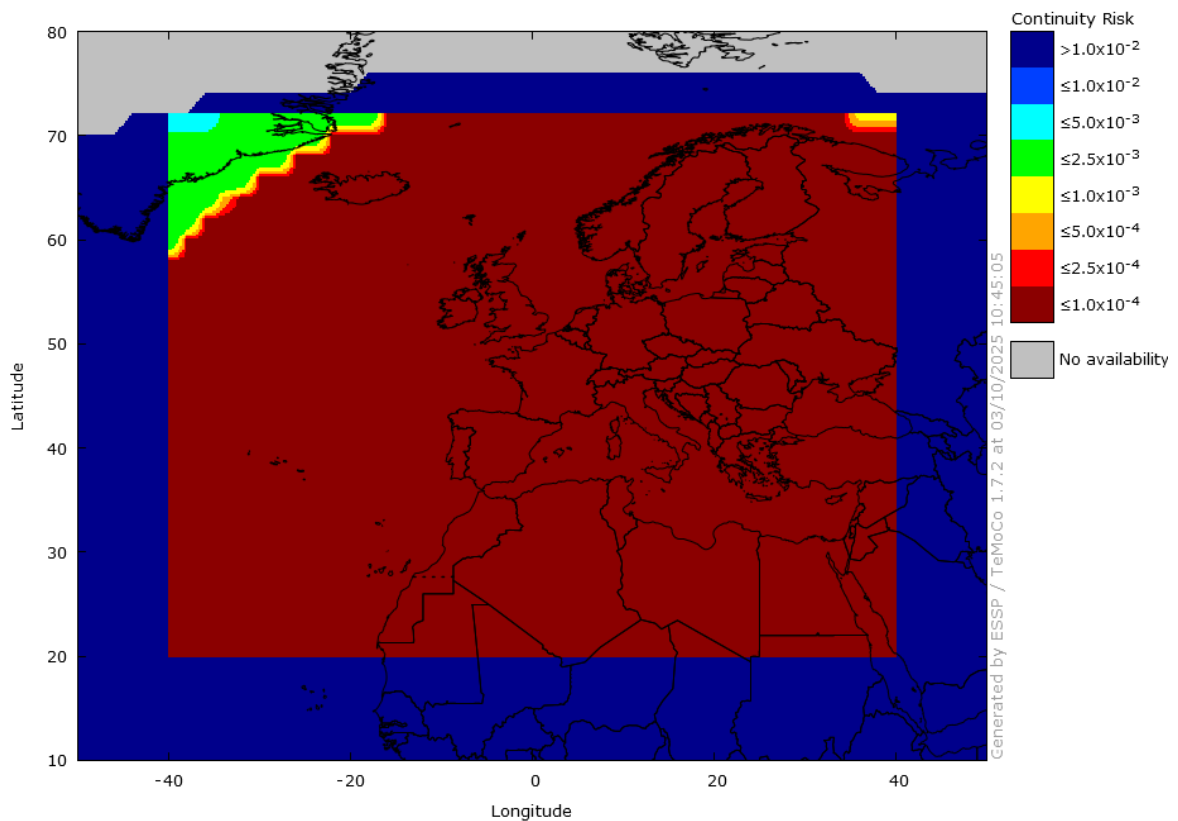
Figure 7 – EGNOS NPA Continuity over the last 6 months
