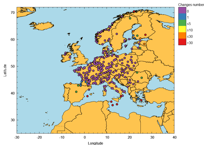
Figure 28 – EGNOS LPV-200 outages in September 2025
