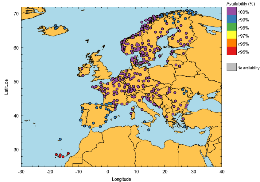
Figure 17 – EGNOS APV-I Availability at airports in September 2025
