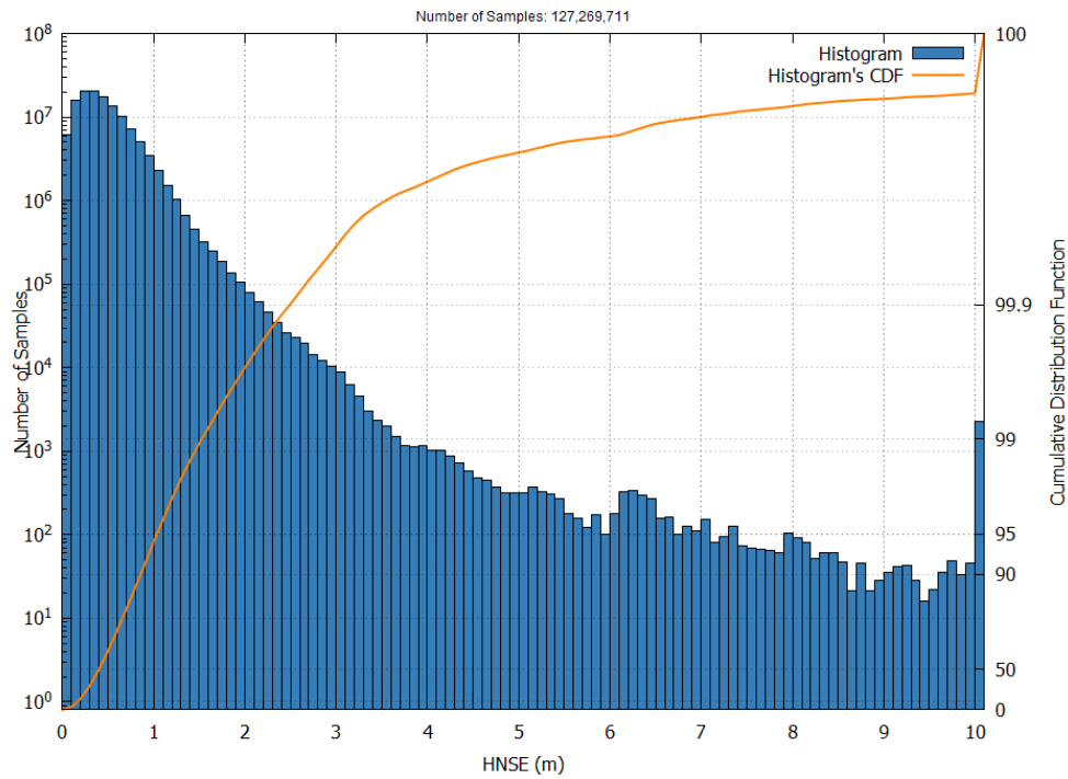
Figure 3 – EGNOS Open Service HNSE Histogram and Cumulative Probability in September 2025
