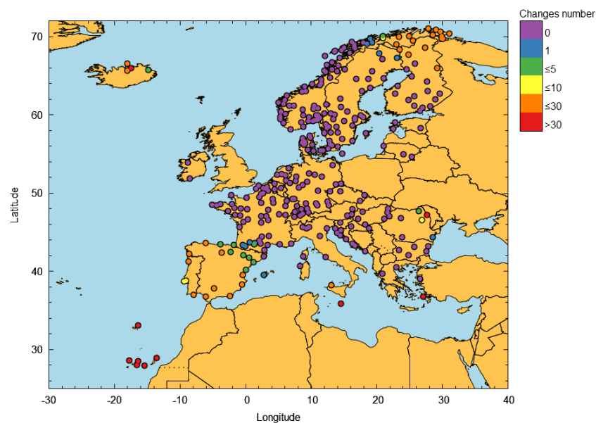
Figure 18 – EGNOS APV-I outages in September 2025
