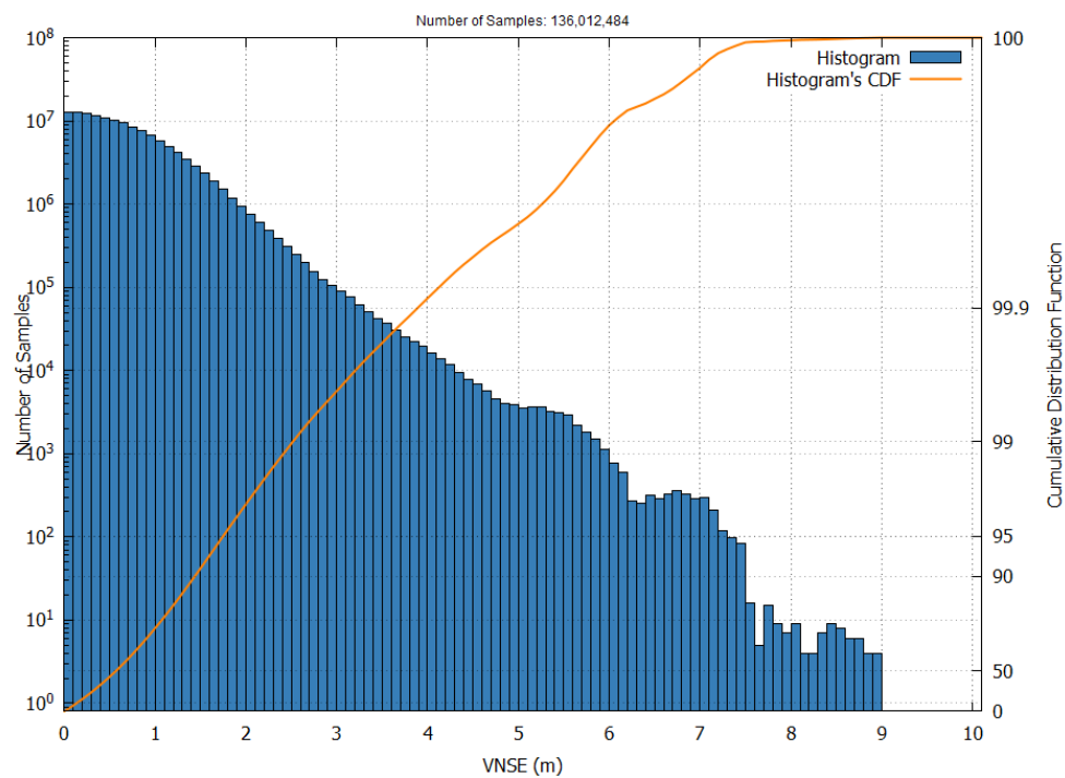
Figure 25 – EGNOS LPV-200 VNSE Histogram and Cumulative Probability in September 2025
