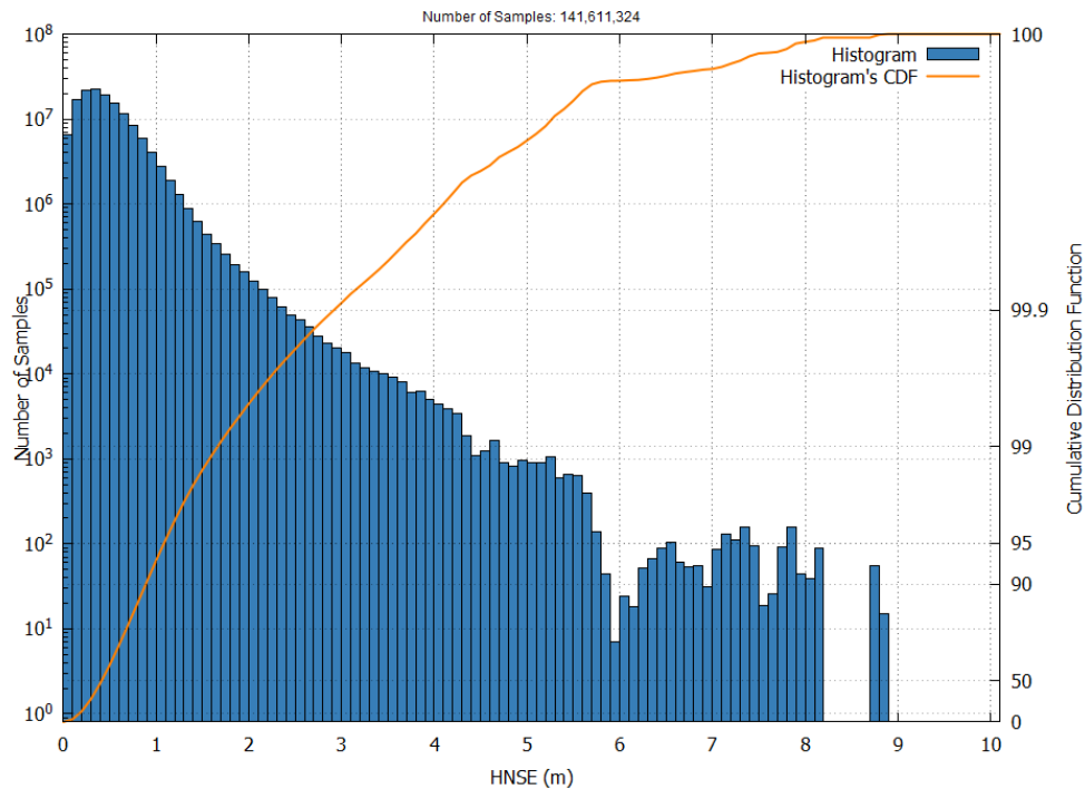
Figure 15 – EGNOS APV-I HNSE Histogram and Cumulative Probability in September 2025
