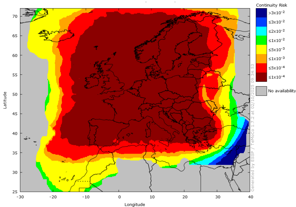
Figure 21 – EGNOS LPV-200 Continuity 2 in September 2025
