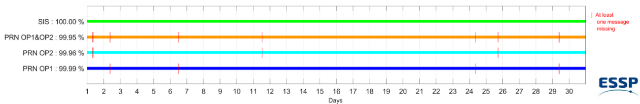
Figure 1 - EGNOS SIS & PRN Availability for September 2025
