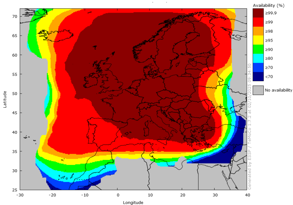
Figure 19 – EGNOS LPV-200 Availability in September 2025
