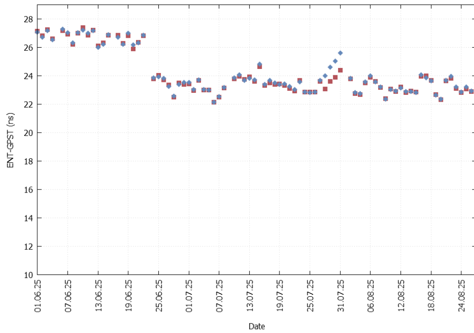
Figure 30 – ENT-GPS offset evolution from June to August 2025 (red PRN 123; blue PRN 136)
