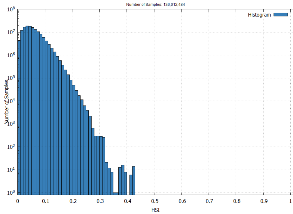
Figure 22 – EGNOS LPV-200 Horizontal Safety Index in September 2025
