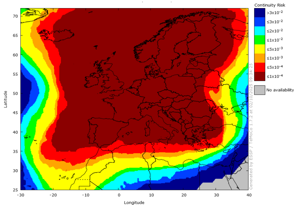
Figure 12 – EGNOS APV-I Continuity in September 2025
