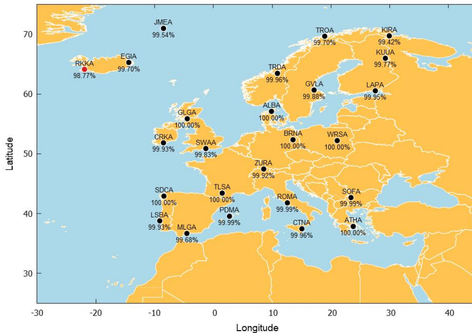
Figure 5 – EGNOS Open Service Availability at reference stations in September 2025
