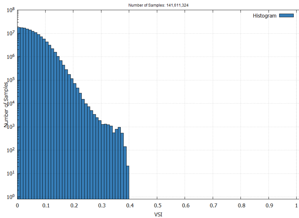
Figure 14 – EGNOS APV-I Vertical Safety Index in September 2025
