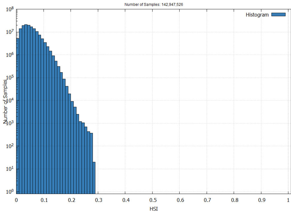
Figure 22 – EGNOS LPV-200 Horizontal Safety Index in July 2025
