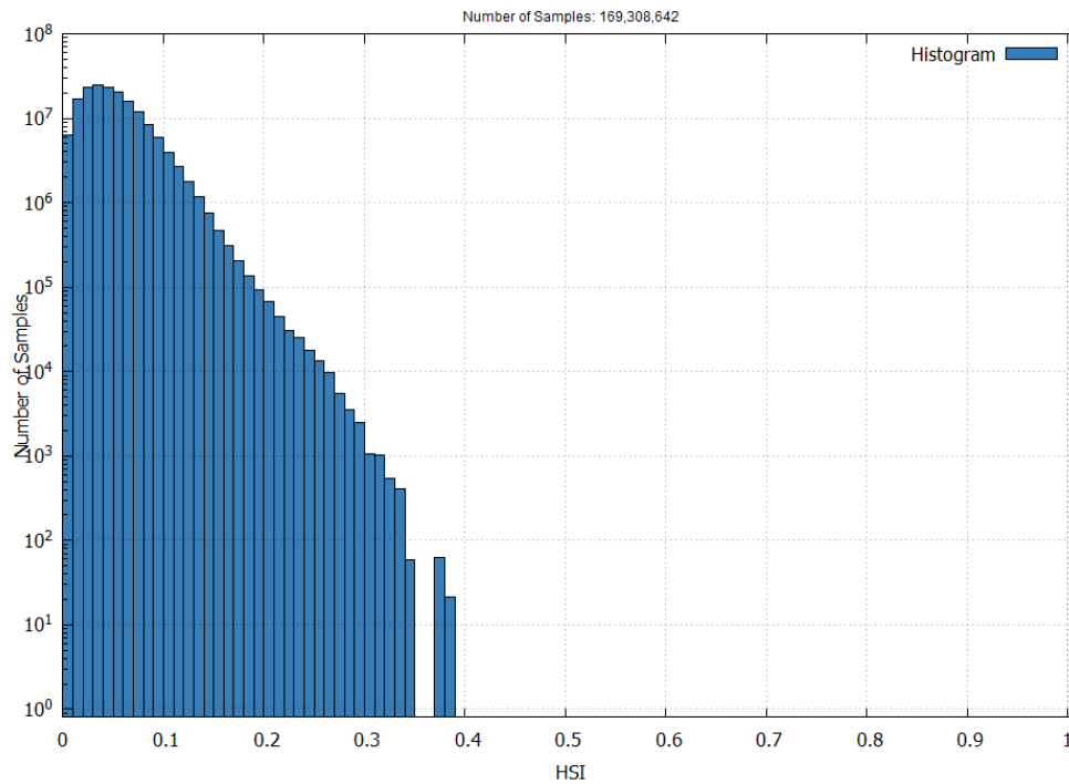
Figure 8 – EGNOS NPA Horizontal Safety Index in July 2025
