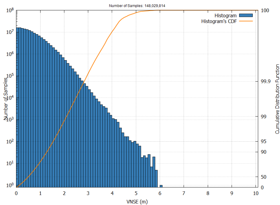
Figure 16 – EGNOS APV-I VNSE Histogram and Cumulative Probability in July 2025
