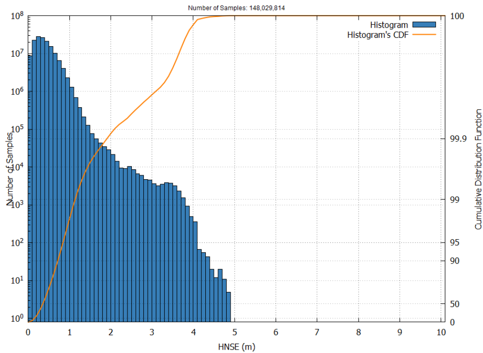
Figure 15 – EGNOS APV-I HNSE Histogram and Cumulative Probability in July 2025
