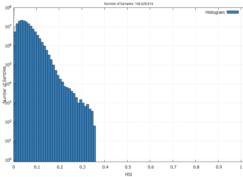
Figure 13 – EGNOS APV-I Horizontal Safety Index in July 2025
