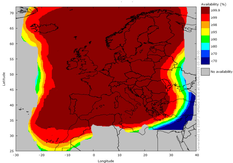
Figure 19 – EGNOS LPV-200 Availability in July 2025
