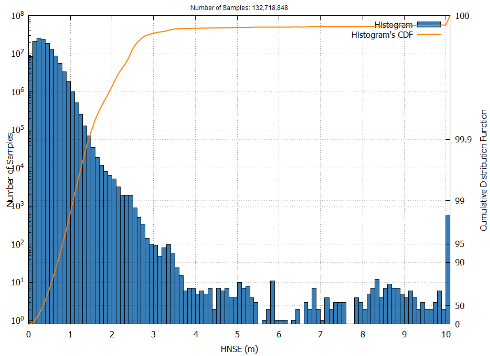
Figure 3 – EGNOS Open Service HNSE Histogram and Cumulative Probability in July 2025
