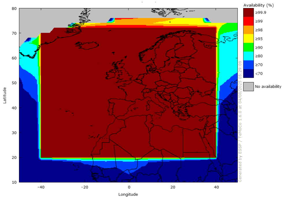
Figure 6 – EGNOS NPA Availability in July 2025
