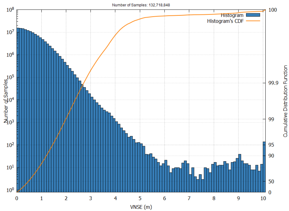
Figure 4 – EGNOS Open Service VNSE Histogram and Cumulative Probability in July 2025
