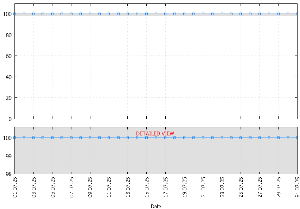
Figure 29 – EGNOS Time Service Availability in July 2025
