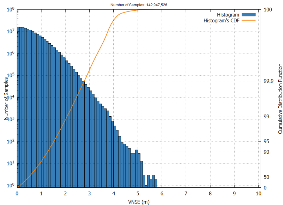
Figure 25 – EGNOS LPV-200 VNSE Histogram and Cumulative Probability in July 2025
