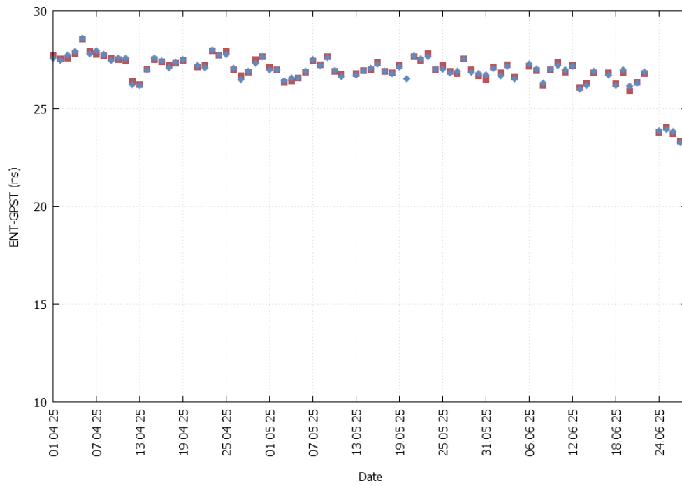
Figure 30 – ENT-GPS offset evolution from April 2025 to June 2025 (red PRN 123; blue PRN 136)
