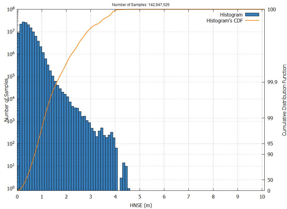
Figure 24 – EGNOS LPV-200 HNSE Histogram and Cumulative Probability in July 2025
