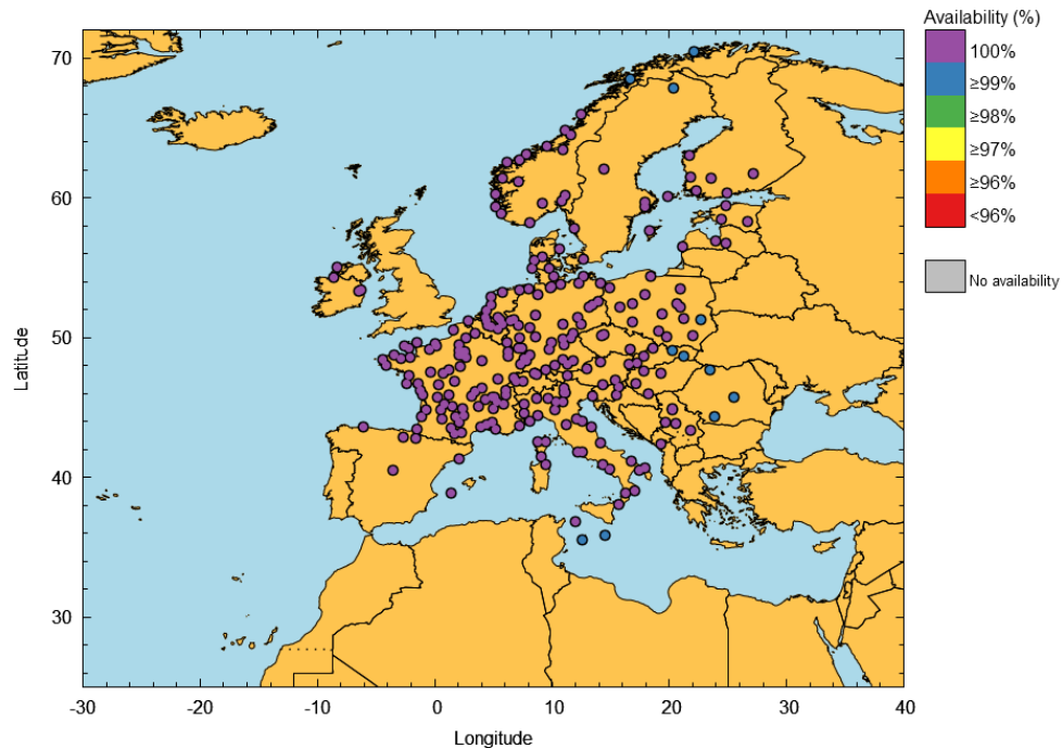
Figure 27 – EGNOS LPV-200 Availability at airports in July 2025
