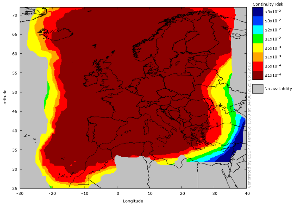
Figure 21 – EGNOS LPV-200 Continuity 2 in July 2025
