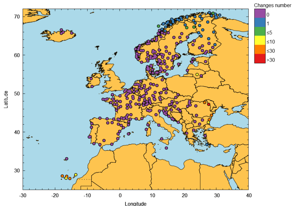
Figure 18 – EGNOS APV-I outages in July 2025
