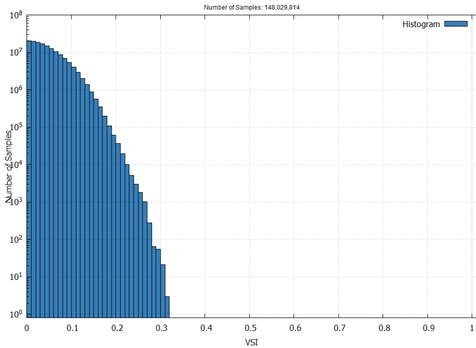
Figure 14 – EGNOS APV-I Vertical Safety Index in July 2025
