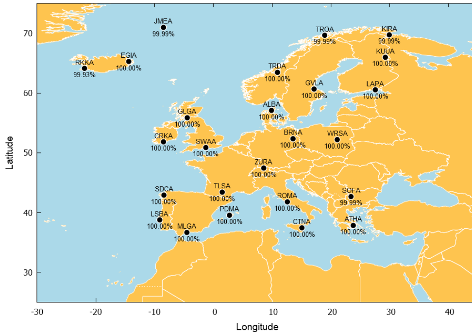
Figure 5 – EGNOS Open Service Availability at reference stations in July 2025
