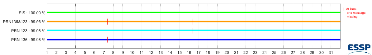
Figure 1 - EGNOS SIS & PRN Availability for July 2025
