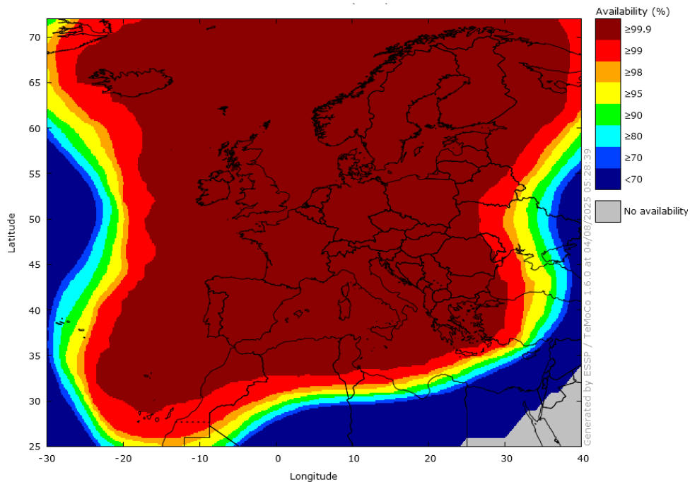
Figure 10 – EGNOS APV-I Availability in July 2025
