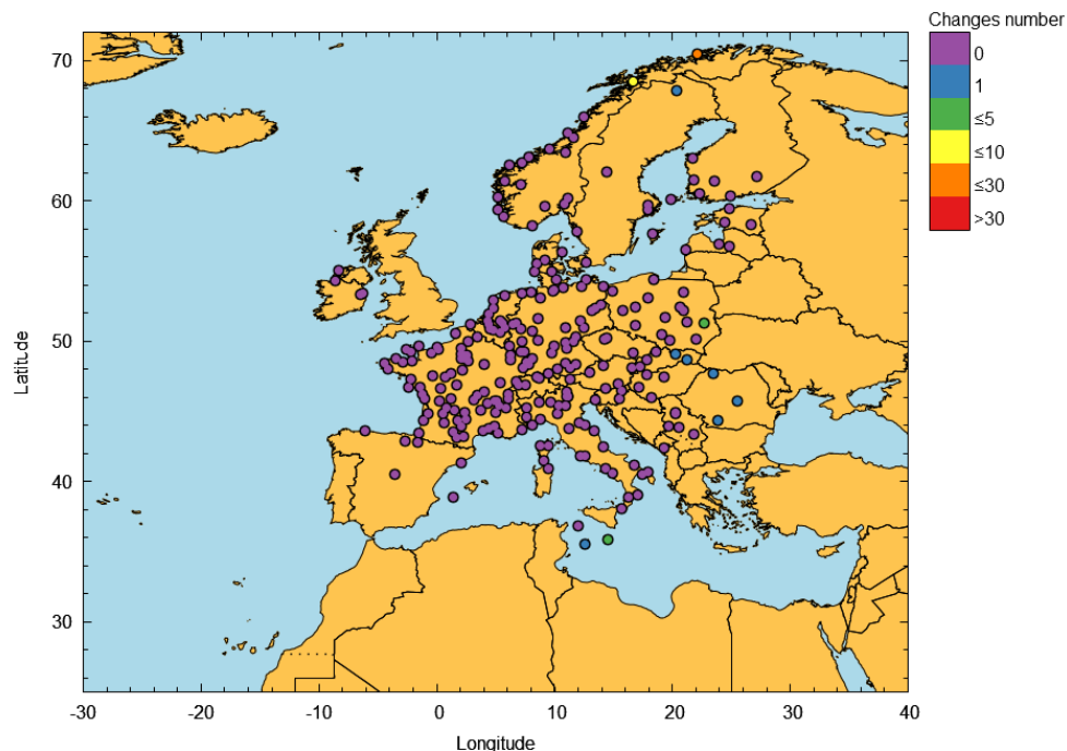
Figure 28 – EGNOS LPV-200 outages in July 2025
