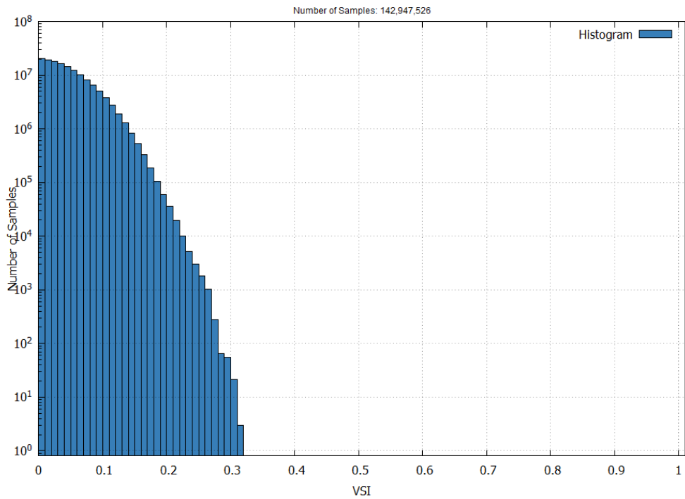
Figure 23 – EGNOS LPV-200 Vertical Safety Index in July 2025
