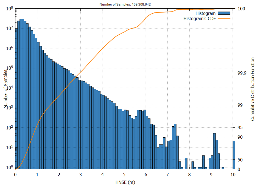
Figure 9 – EGNOS NPA HNSE Histogram and Cumulative Probability in July 2025
