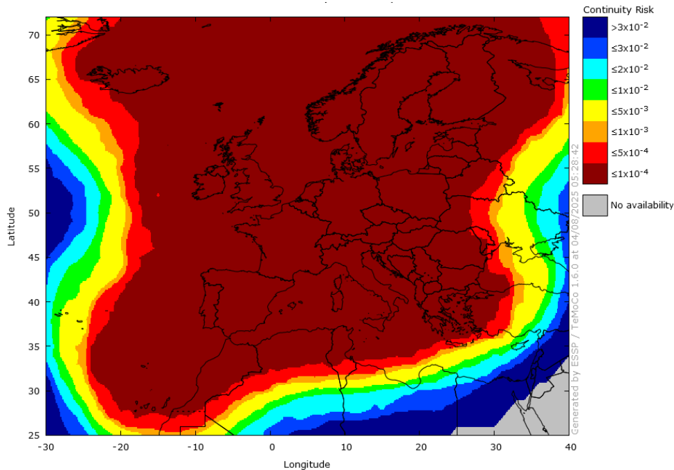
Figure 12 – EGNOS APV-I Continuity in July 2025
