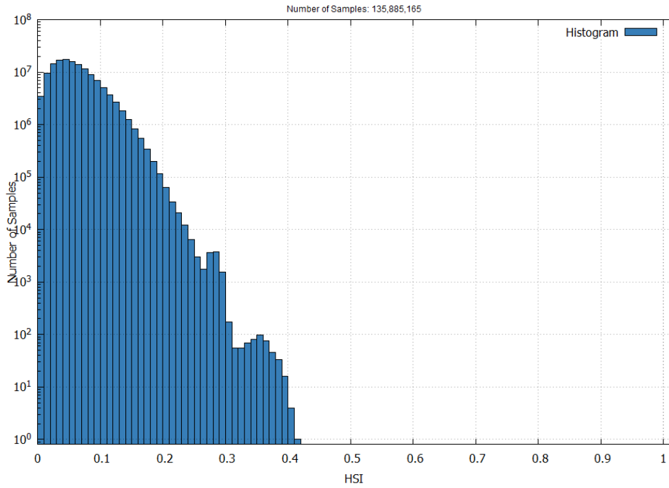
Figure 22 – EGNOS LPV-200 Horizontal Safety Index in April 2025
