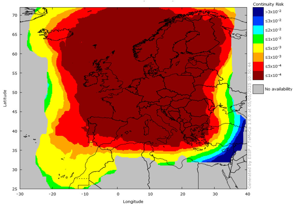
Figure 21 – EGNOS LPV-200 Continuity 2 in April 2025
