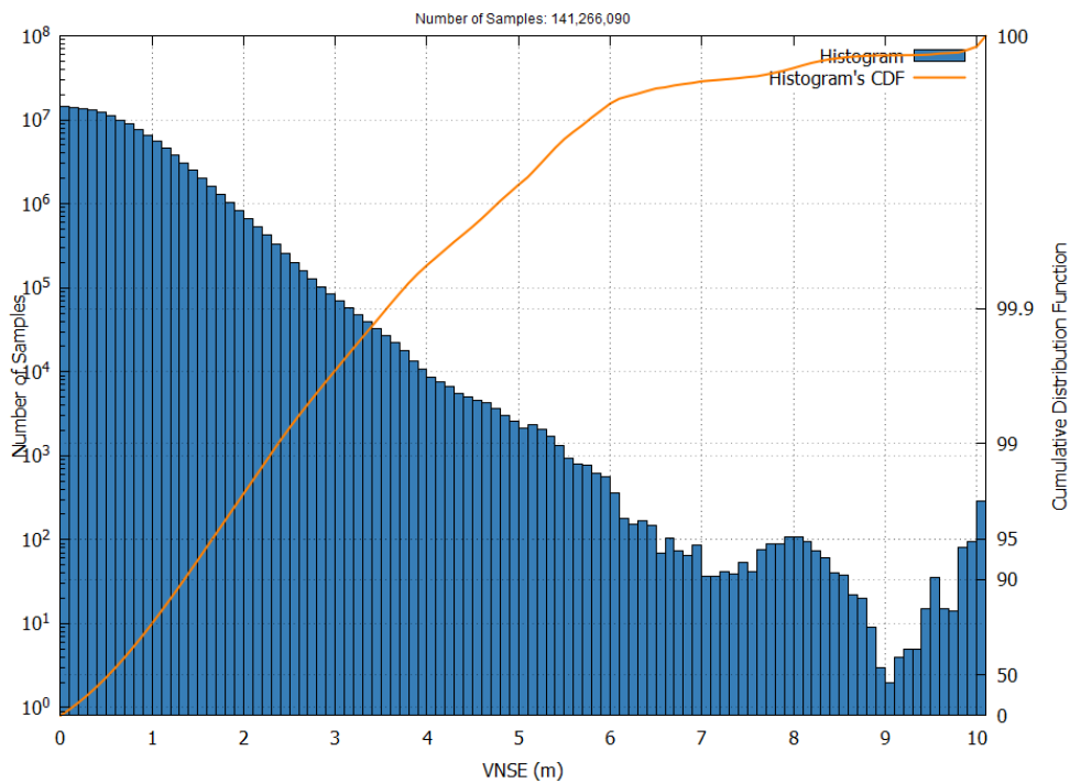
Figure 16 – EGNOS APV-I VNSE Histogram and Cumulative Probability in April 2025
