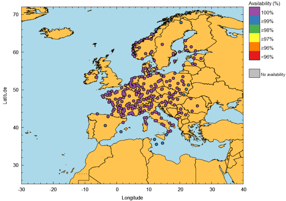
Figure 27 – EGNOS LPV-200 Availability at airports in April 2025
