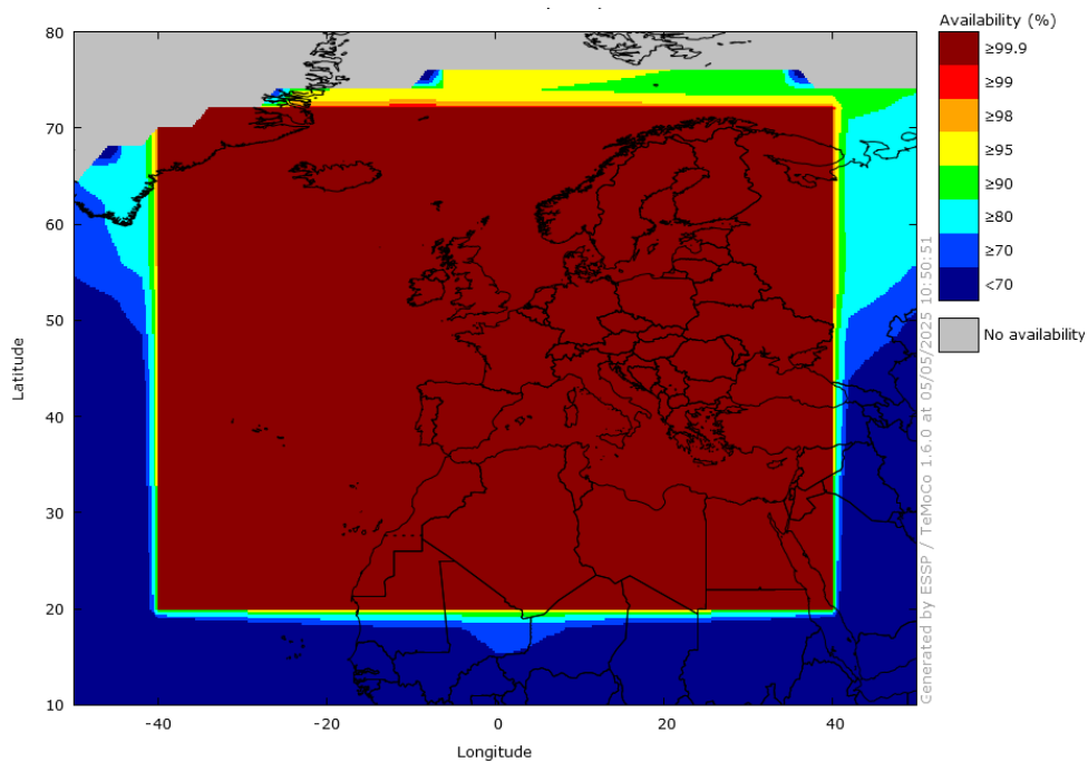
Figure 6 – EGNOS NPA Availability in April 2025
