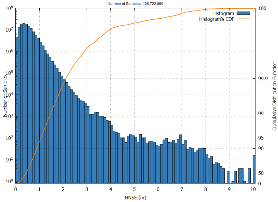
Figure 3 – EGNOS Open Service HNSE Histogram and Cumulative Probability in April 2025
