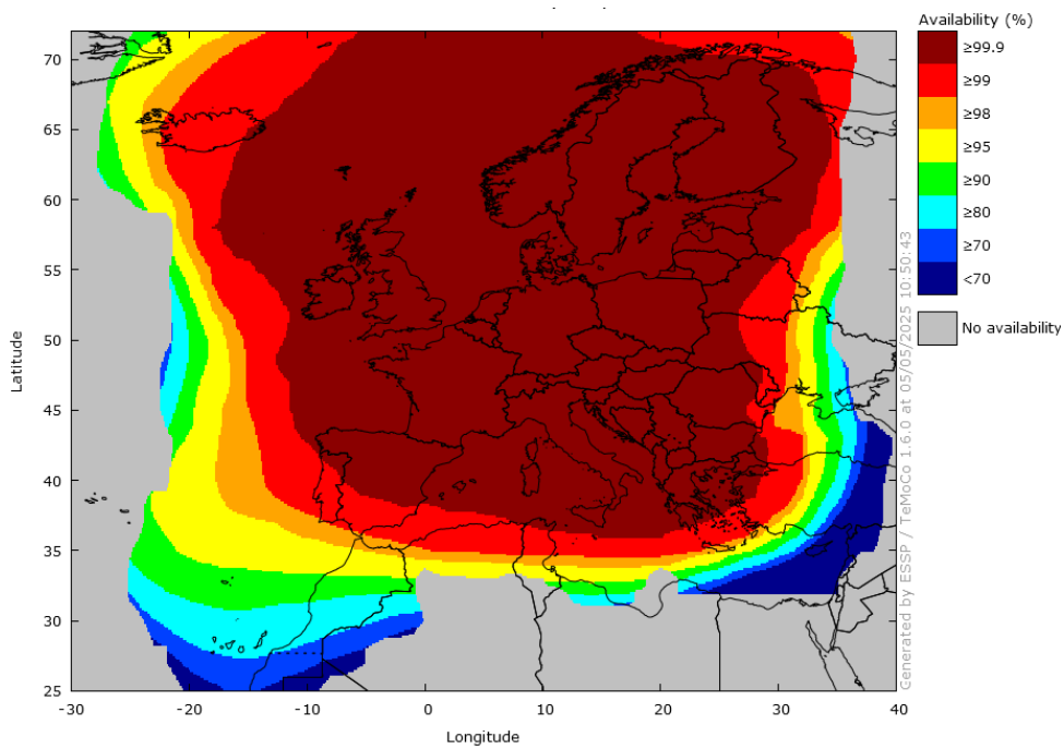
Figure 19 – EGNOS LPV-200 Availability in April 2025
