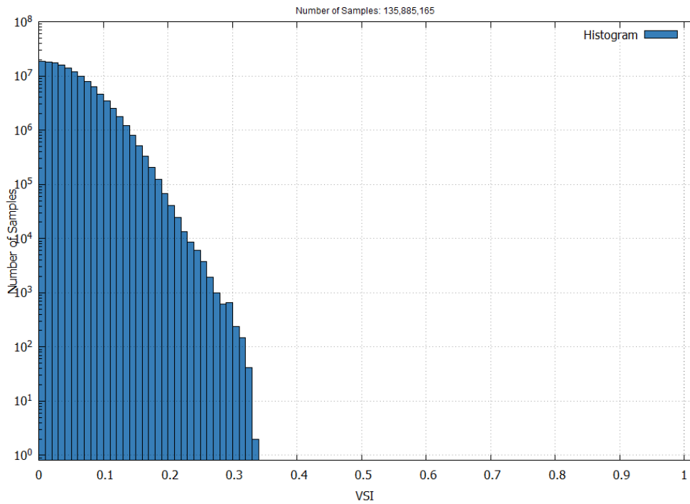
Figure 23 – EGNOS LPV-200 Vertical Safety Index in April 2025
