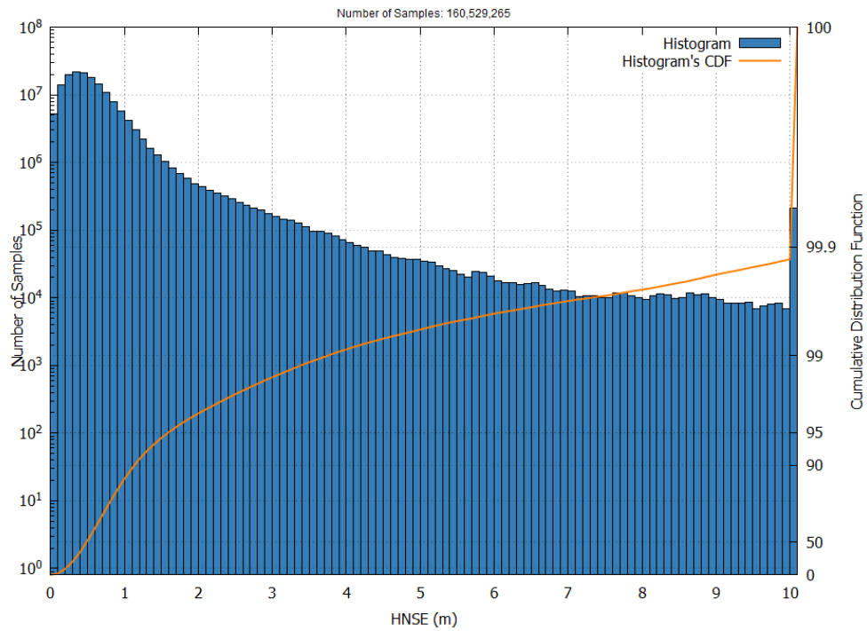
Figure 9 – EGNOS NPA HNSE Histogram and Cumulative Probability in April 2025
