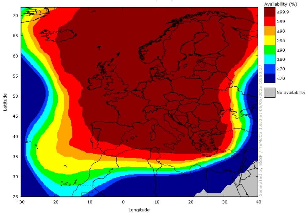
Figure 10 – EGNOS APV-I Availability in April 2025
