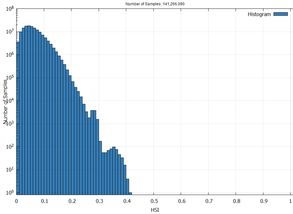
Figure 13 – EGNOS APV-I Horizontal Safety Index in April 2025
