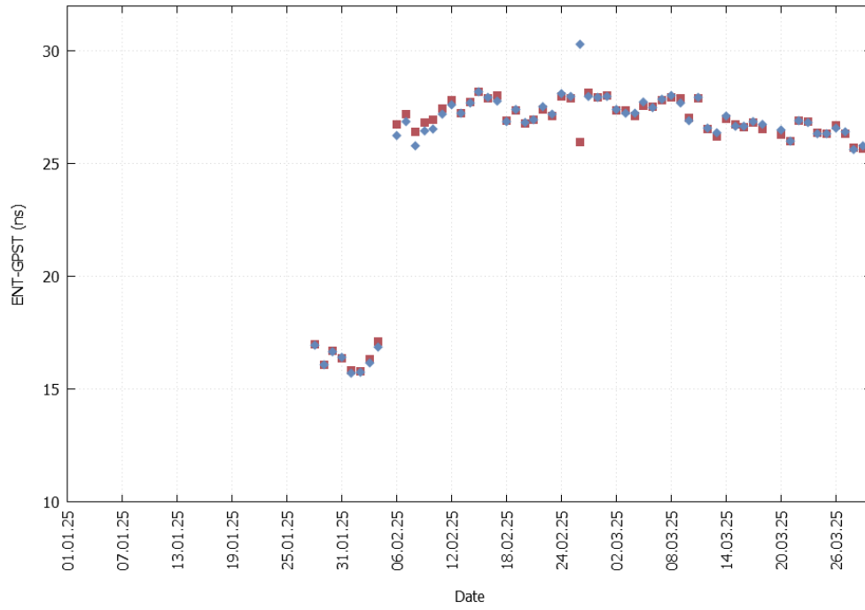
Figure 30 – ENT-GPS offset evolution from January to March 2025 (red PRN 123; blue PRN 136)
