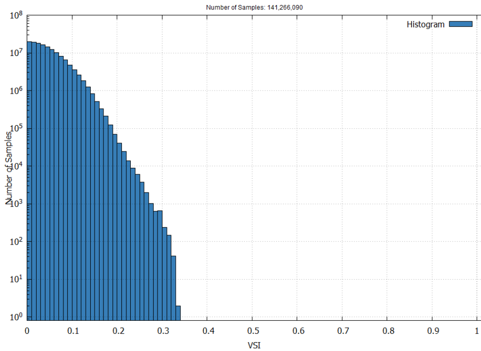
Figure 14 – EGNOS APV-I Vertical Safety Index in April 2025
