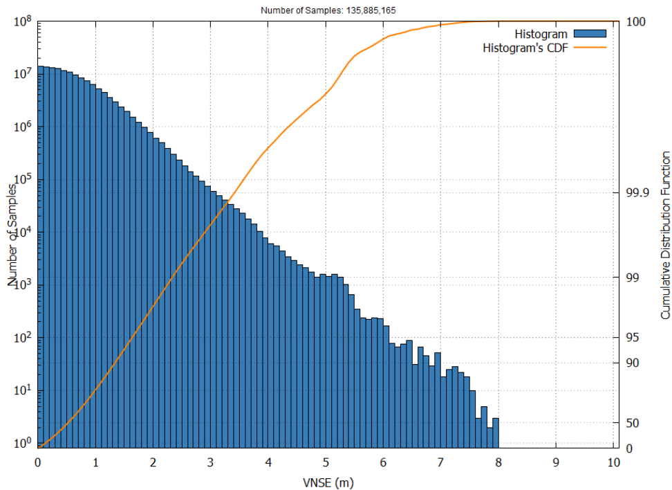
Figure 25 – EGNOS LPV-200 VNSE Histogram and Cumulative Probability in April 2025
