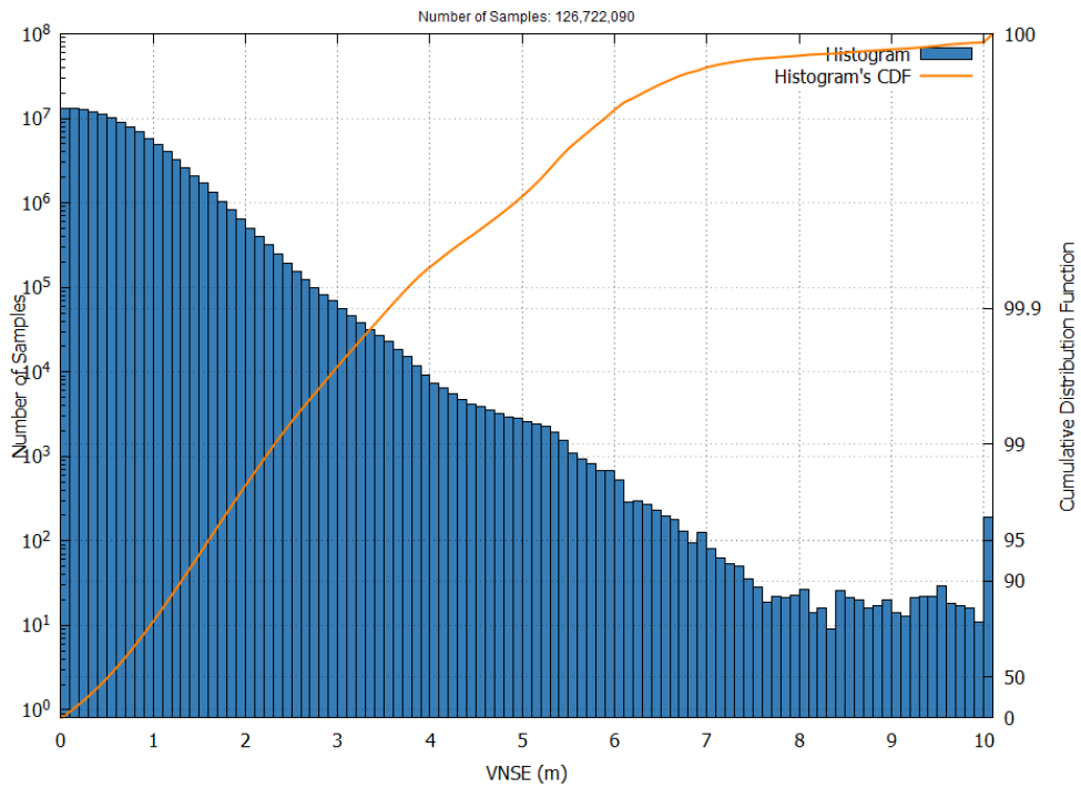
Figure 4 – EGNOS Open Service VNSE Histogram and Cumulative Probability in April 2025
