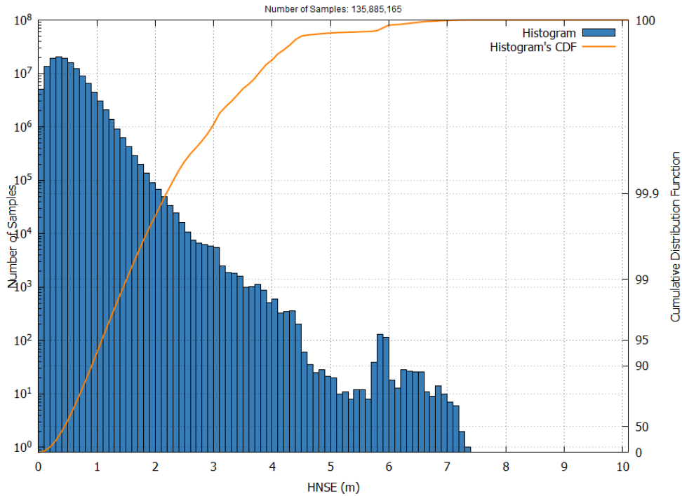
Figure 24 – EGNOS LPV-200 HNSE Histogram and Cumulative Probability in April 2025
