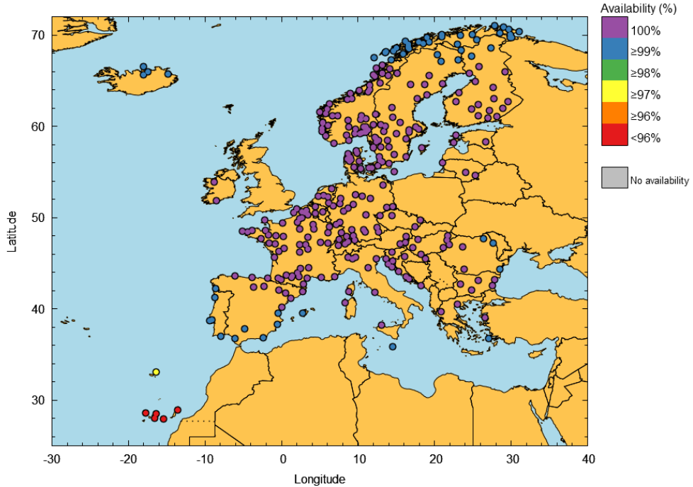
Figure 17 – EGNOS APV-I Availability at airports in April 2025
