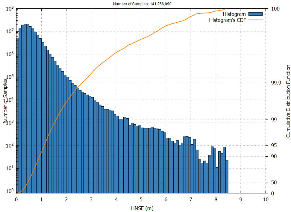
Figure 15 – EGNOS APV-I HNSE Histogram and Cumulative Probability in April 2025
