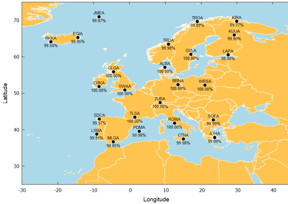
Figure 5 – EGNOS Open Service Availability at reference stations in April 2025
