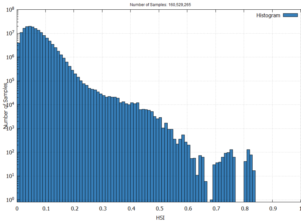
Figure 8 – EGNOS NPA Horizontal Safety Index in April 2025
