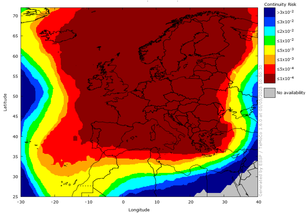
Figure 12 – EGNOS APV-I Continuity in April 2025
