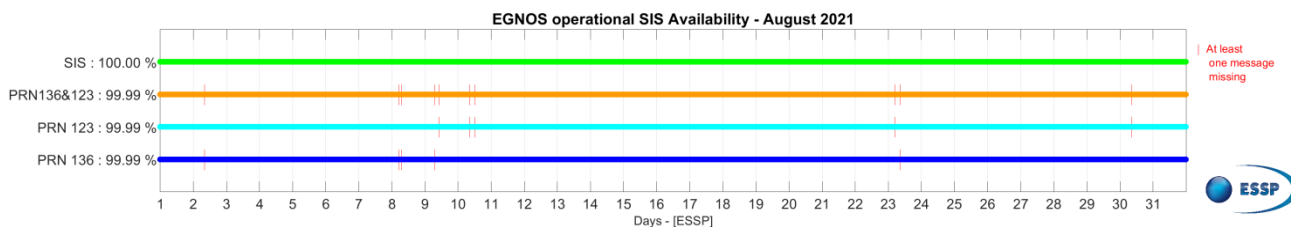
Figure 1 – EGNOS SIS & PRN Availability for August 2021
