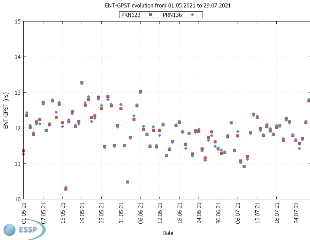
Figure 29 – ENT-GPS offset evolution
