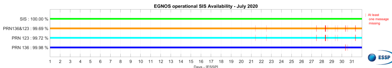
Figure 1 – EGNOS SIS & PRN Availability for July 2020
