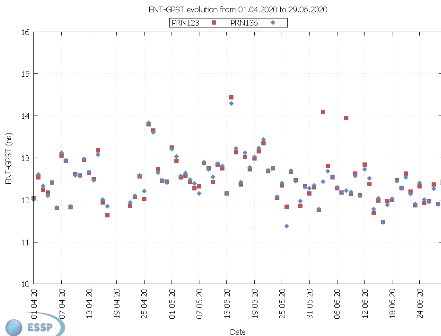
Figure 30 – ENT-GPS offset evolution
