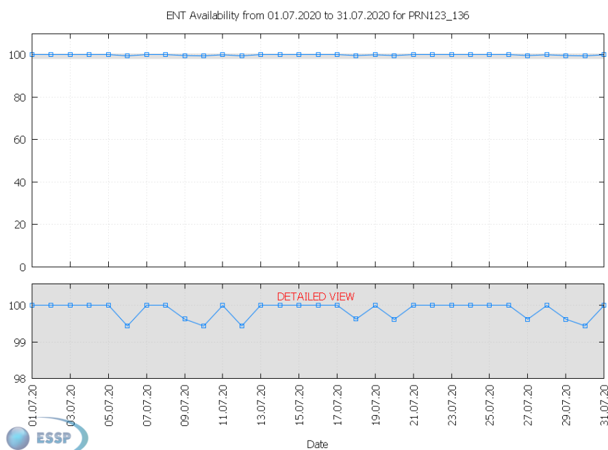
Figure 29 – EGNOS Time Service availability
